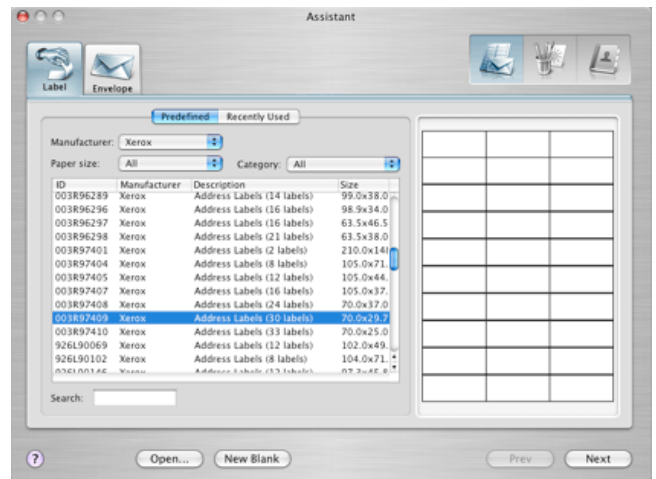
Label Assistant
