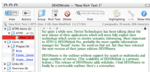
DEVONnote
