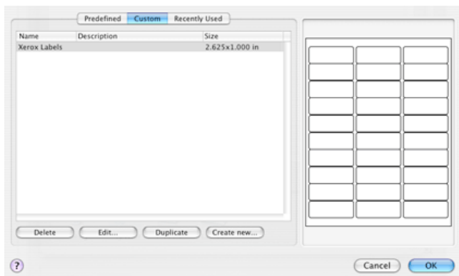
Custom Labels
