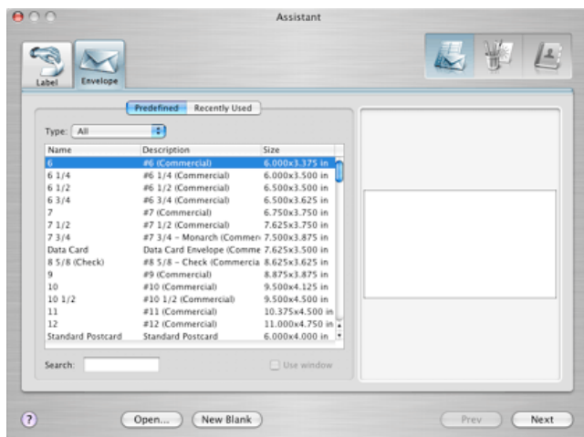
Envelope Assistant
