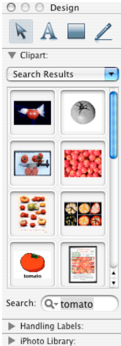
Design Palette
