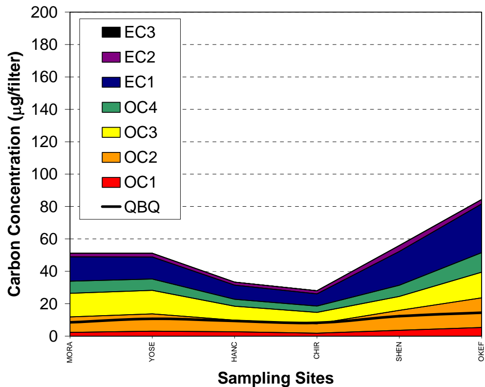
Figure 3-6. Average carbon concentration from the quartz-fiber backup filter (QBQ) compared with concurrent quartz-fiber front filter (QF) carbon fraction concentrations for six sites in the IMPROVE network.
