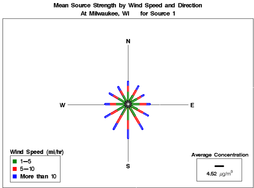
Figure I-2. Pollution Rose for Milwaukee, Wisconsin, Source 1 - Coal Combustion (Ni).
