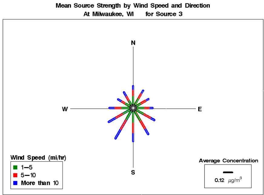
Figure I-14 Pollution Rose for Milwaukee, Wisconsin, Source 3 - Crustal.
