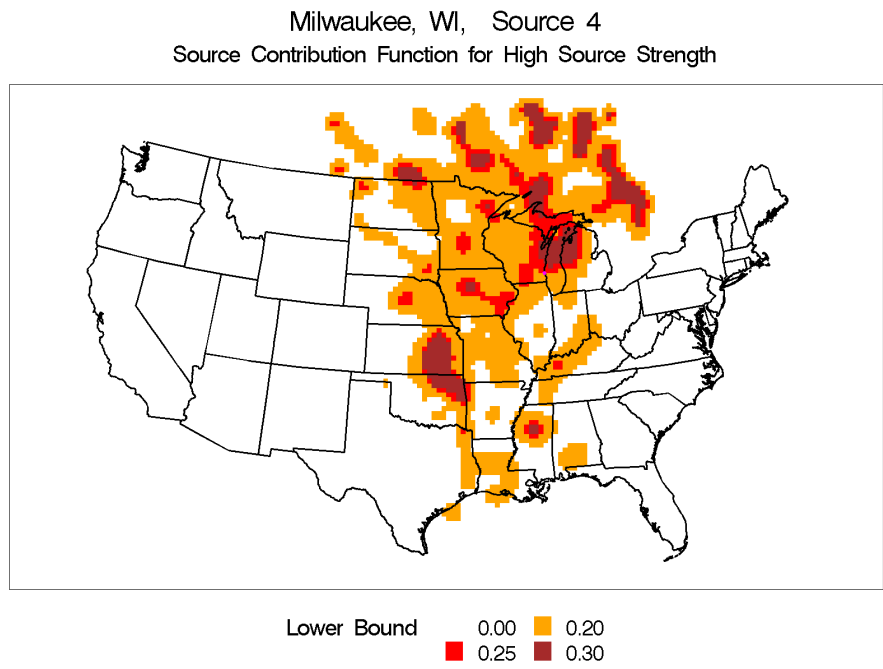
Figure I-21 Source Contribution Contour Plot for Milwaukee, Wisconsin, Source 4 - Chlorine Sources.
