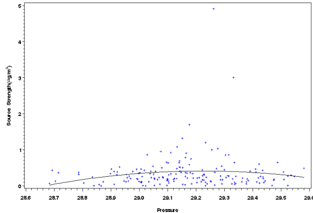
Figure I-42 Scatter Plot of Source Strength Versus Mean Daily Temperature (Rows 1 and 2) and Pressure (bottom) for Milwaukee, Wisconsin, Source 7 - Vegetative Burning and Fireworks.
