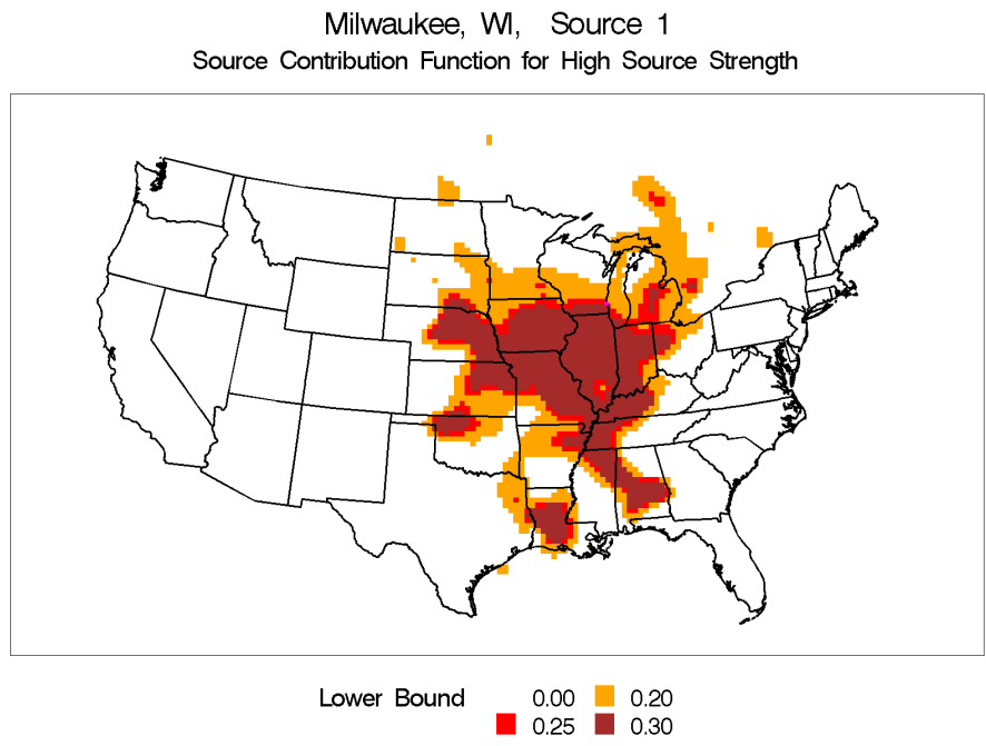
Figure I-3 Source Contribution Contour Plot for Milwaukee, Wisconsin, Source 1 - Coal Combustion (Ni).
