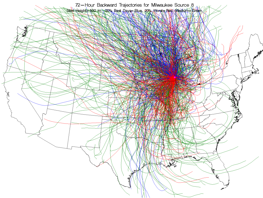
Figure I-47 Back Trajectories Color Coded by Source Strength Category for Milwaukee, Wisconsin, Source 8 - Industrial Diesel and Sulfate Mix.
