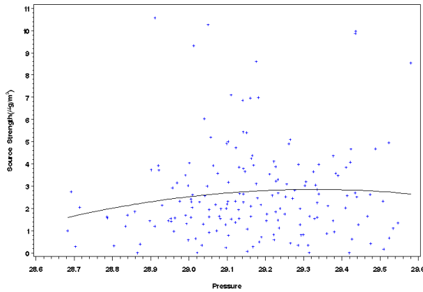
Figure I-24 Scatter Plot of Source Strength Versus Mean Daily Temperature (Rows 1 and 2) and Pressure (bottom) for Milwaukee, Wisconsin, Source 4 - Chlorine Sources.
