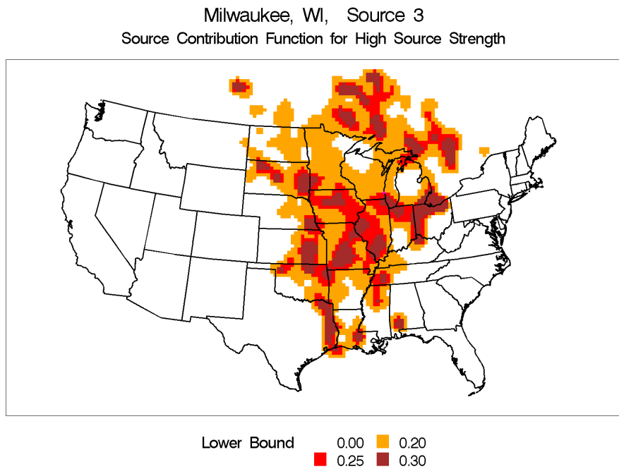
Figure I-15 Source Contribution Contour Plot for Milwaukee, Wisconsin, Source 3 - Crustal.
