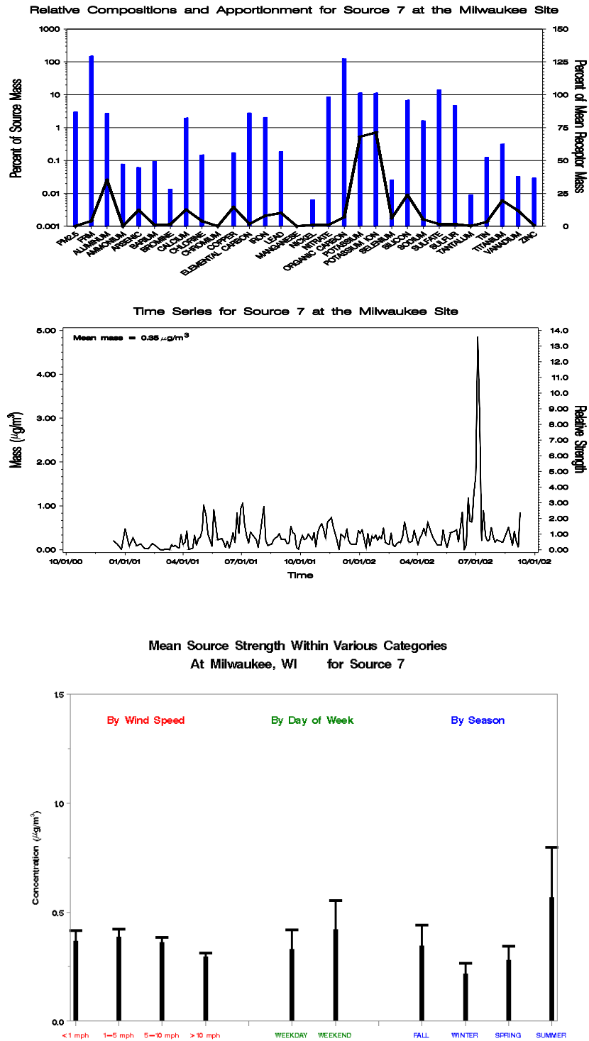
Figure I-37 Profile Plot (Top), Time Series Plot (Middle), and Bar Charts of the Source Strength Averaged by Wind Speed, Day of Week, and Season (Bottom) for Milwaukee, Wisconsin, Source 7 - Vegetative Burning and Fireworks.
