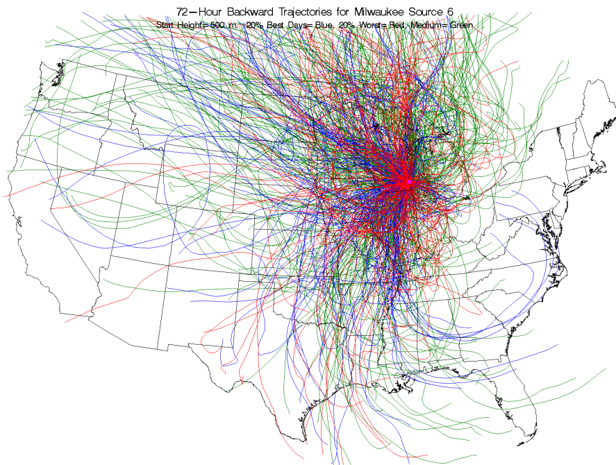
Figure I-35 Back Trajectories Color Coded by Source Strength Category for Milwaukee, Wisconsin, Source 6 - Crustal Related Events.
