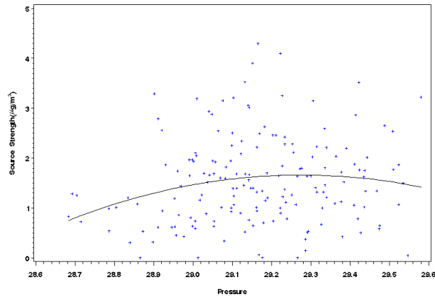
Figure I-12 Scatter Plot of Source Strength Versus Mean Daily Temperature (Rows 1 and 2) and Pressure (bottom) for Milwaukee, Wisconsin, Source 2 - Mobile Sources.
