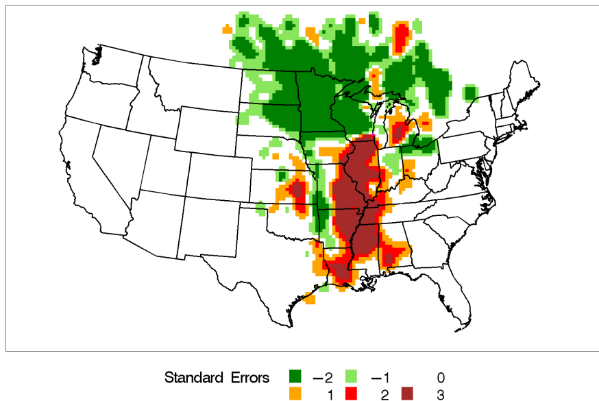
Figure I-40 Incremental Probability Contour Plot for Milwaukee, Wisconsin, Source 7 - Vegetative Burning and Fireworks.
