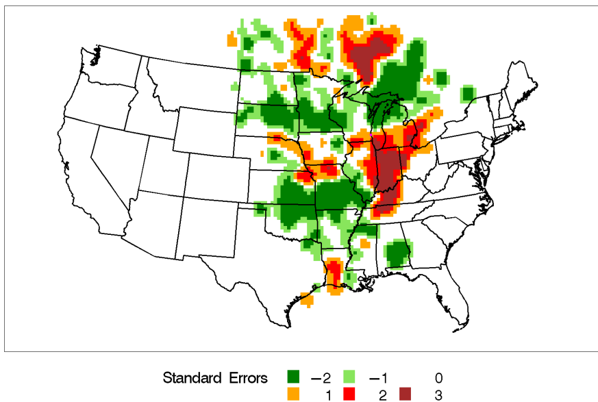
Milwaukee, WI, Source 6 Incremental Probability for High Source Strength
