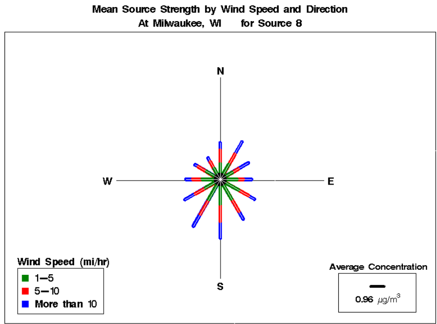
Figure I-44 Pollution Rose for Milwaukee, Wisconsin, Source 8 - Industrial Diesel and Sulfate Mix.
