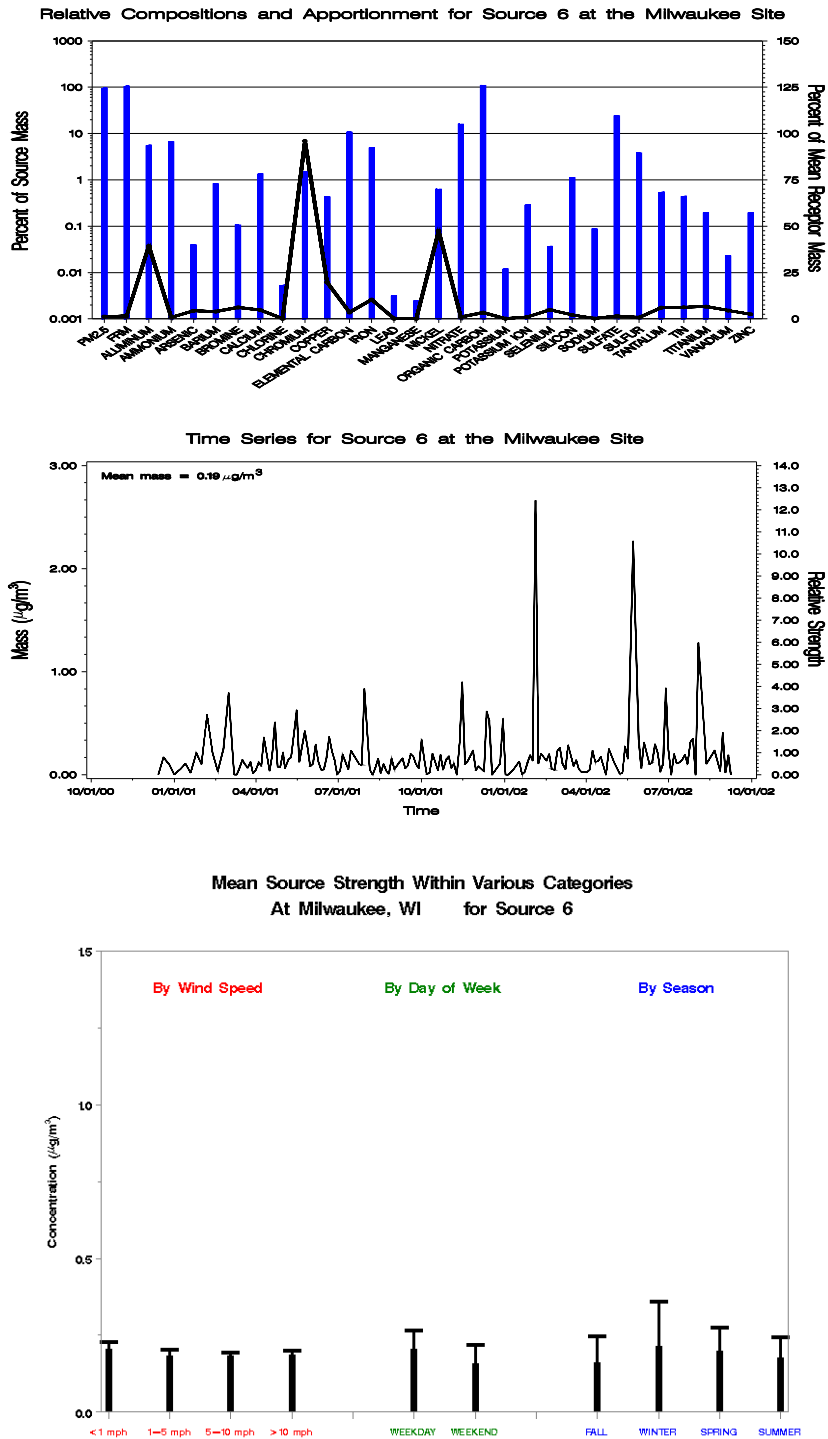
Figure I-31 Profile Plot (Top), Time Series Plot (Middle), and Bar Charts of the Source Strength Averaged by Wind Speed, Day of Week, and Season (Bottom) for Milwaukee, Wisconsin, Source 6 - Crustal Related Events.
