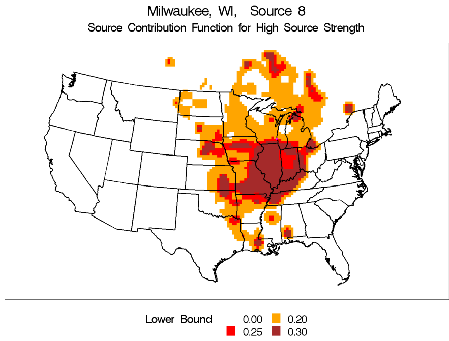
Figure I-45 Source Contribution Contour Plot for Milwaukee, Wisconsin, Source 8 - Industrial Diesel and Sulfate Mix.
