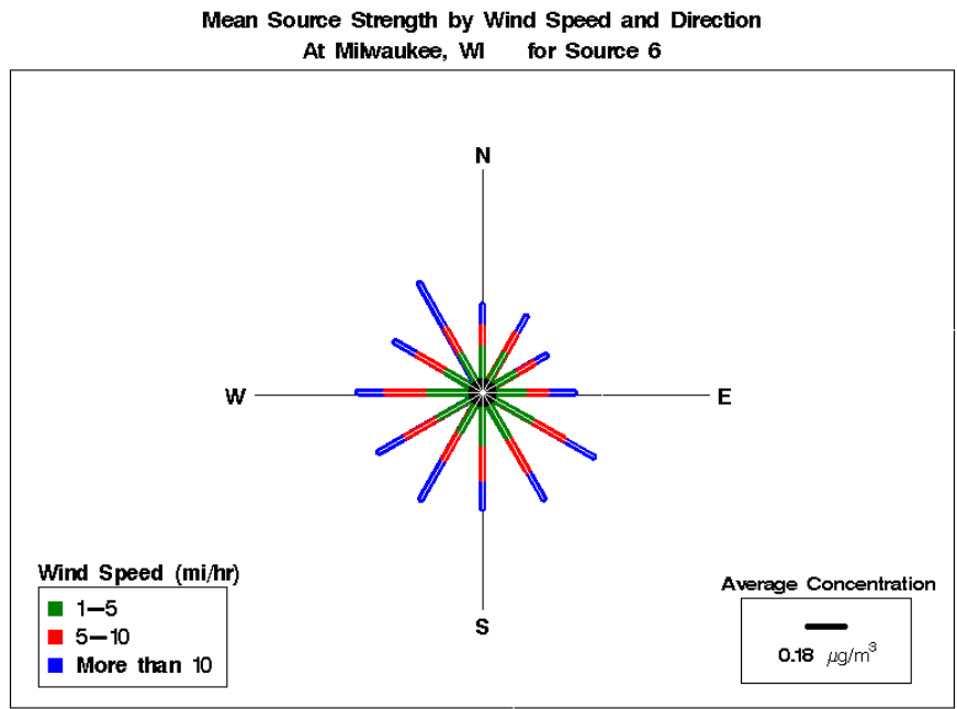
Figure I-32 Pollution Rose for Milwaukee, Wisconsin, Source 6 - Crustal Related Events.
