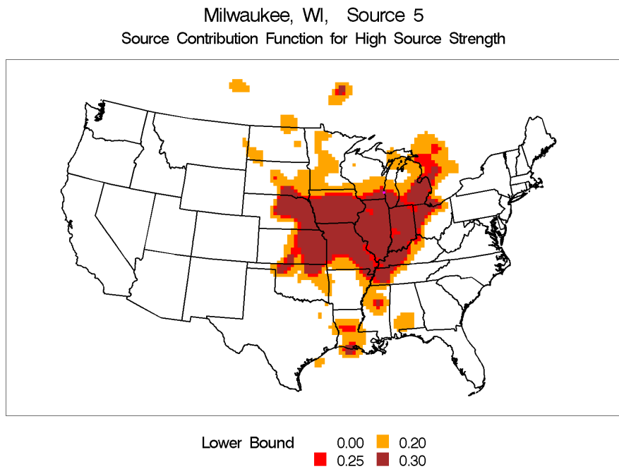
Figure I-27 Source Contribution Contour Plot for Milwaukee, Wisconsin, Source 5 - Ammonium Nitrate.
