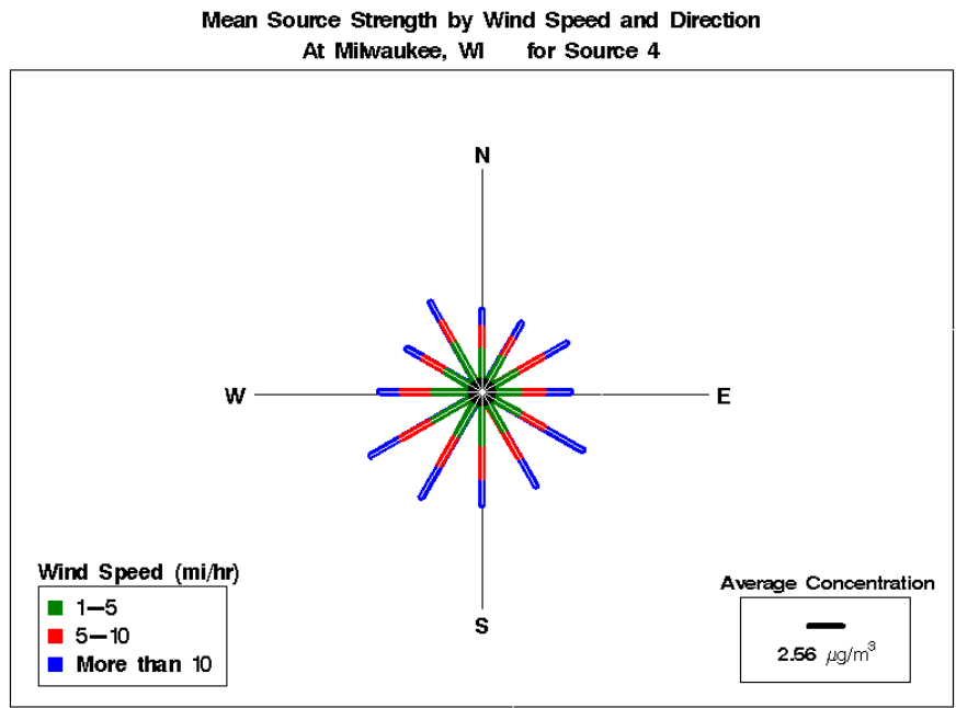
Figure I-20 Pollution Rose for Milwaukee, Wisconsin, Source 4 - Chlorine Sources.
