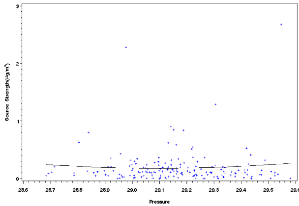
Figure I-36 Scatter Plot of Source Strength Versus Mean Daily Temperature (Rows 1 and 2) and Pressure (bottom) for Milwaukee, Wisconsin, Source 6 - Crustal Related Events.
