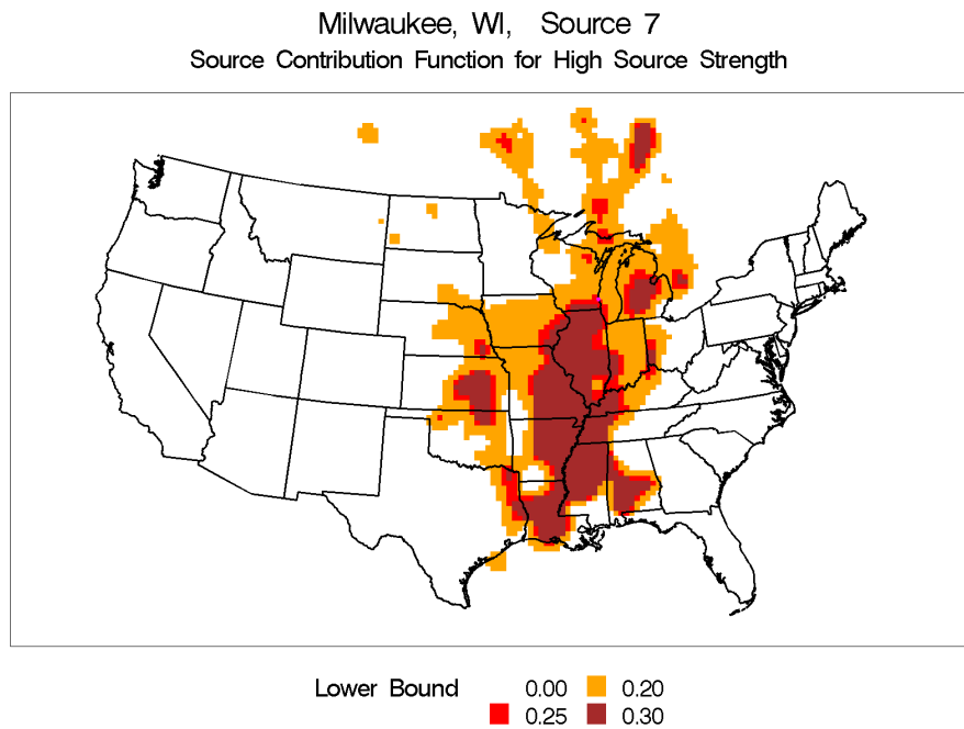
Figure I-39 Source Contribution Contour Plot for Milwaukee, Wisconsin, Source 7 - Vegetative Burning and Fireworks.
