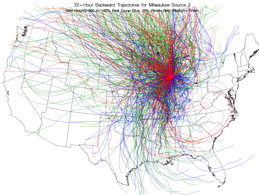
Figure I-11 Back Trajectories Color Coded by Source Strength Category for Milwaukee, Wisconsin, Source 2 - Mobile Sources.
