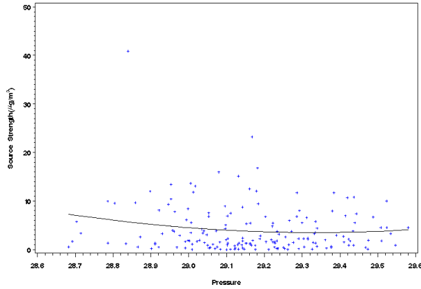
Figure I-30 Scatter Plot of Source Strength Versus Mean Daily Temperature (Rows 1 and 2) and Pressure (bottom) for Milwaukee, Wisconsin, Source 5 - Ammonium Nitrate.
