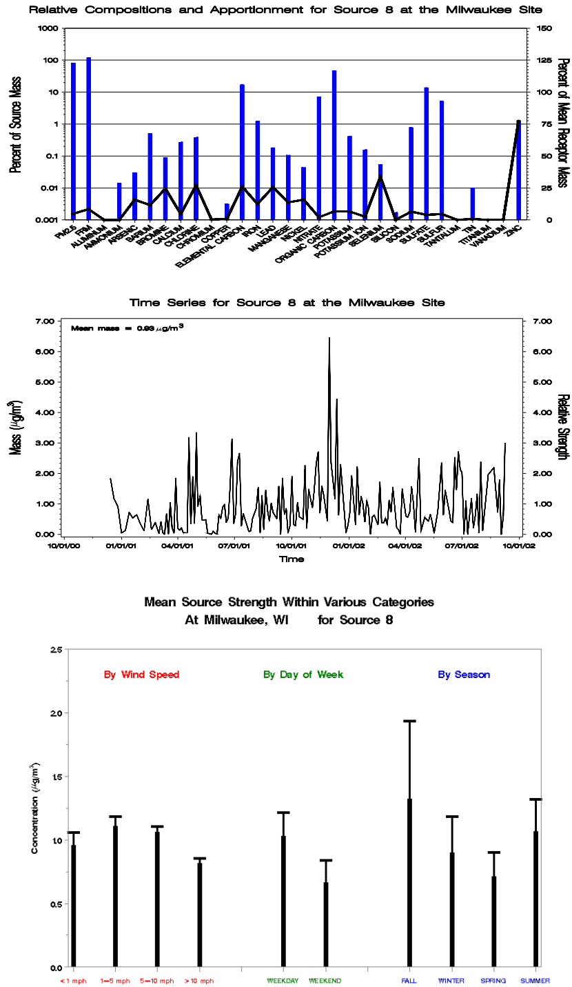
Figure I-43 Profile Plot (Top), Time Series Plot (Middle), and Bar Charts of the Source Strength Averaged by Wind Speed, Day of Week, and Season (Bottom) for Milwaukee, Wisconsin, Source 8 - Industrial Diesel and Sulfate Mix.
