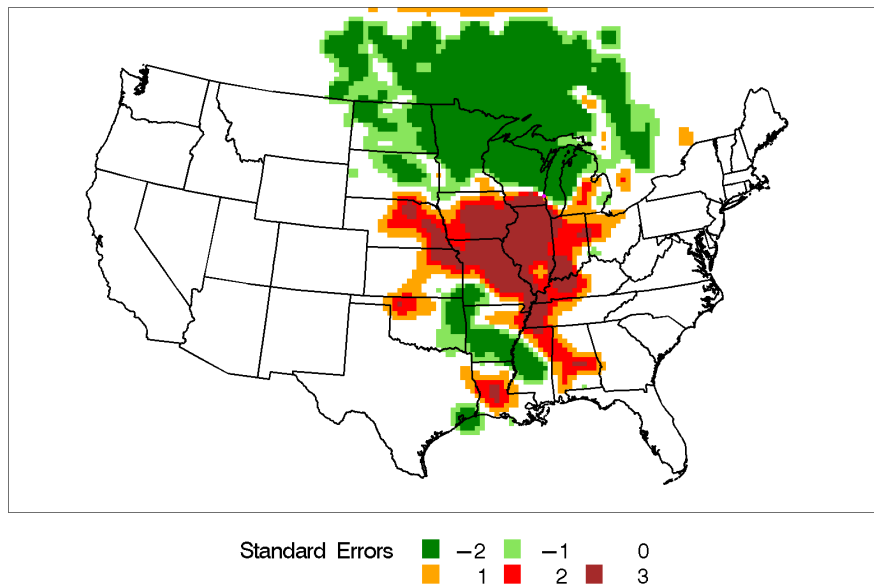
Milwaukee, WI, Source 1 Incremental Probability for High Source Strength
