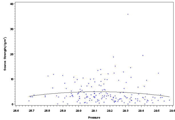
Figure I-6 Scatter Plot of Source Strength Versus Mean Daily Temperature (Rows 1 and 2) and Pressure (bottom) for Milwaukee, Wisconsin, Source 1 - Coal Combustion (Ni).
