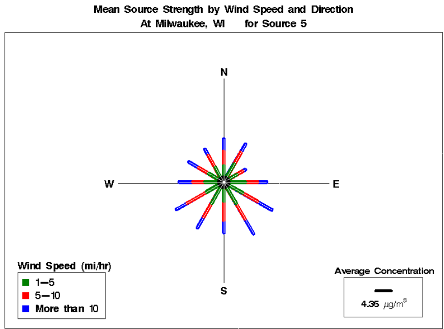
Figure I-26 Pollution Rose for Milwaukee, Wisconsin, Source 5 - Ammonium Nitrate.
