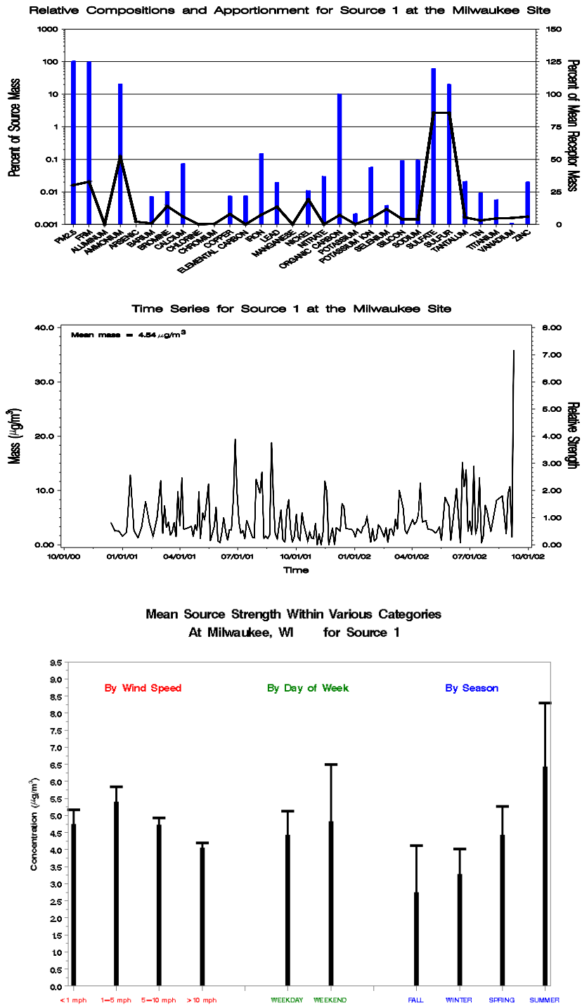
Figure I-1. Profile Plot (Top), Time Series Plot (Middle), and Bar Charts of the Source Strength Averaged by Wind Speed, Day of Week, and Season (Bottom) for Milwaukee, Wisconsin, Source 1 - Coal Combustion (Ni).
