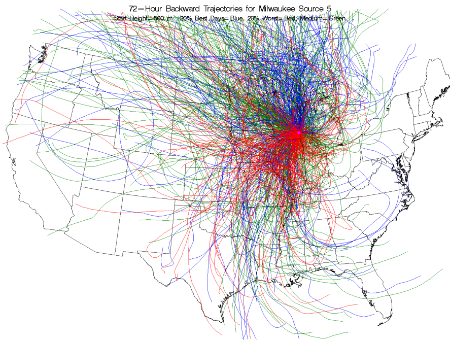
Figure I-29 Back Trajectories Color Coded by Source Strength Category for Milwaukee, Wisconsin, Source 5 - Ammonium Nitrate.
