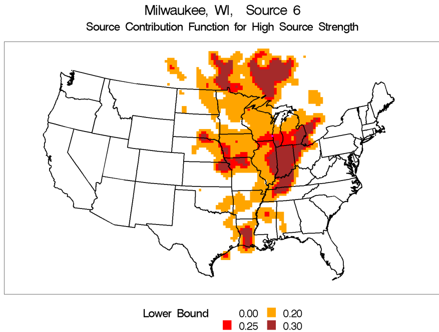
Figure I-33 Source Contribution Contour Plot for Milwaukee, Wisconsin, Source 6 - Crustal Related Events.
