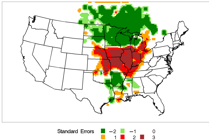
Figure I-28 Incremental Probability Contour Plot for Milwaukee, Wisconsin, Source 5 - Ammonium Nitrate.
