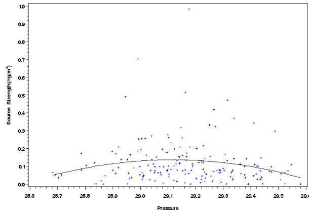
Figure I-18 Scatter Plot of Source Strength Versus Mean Daily Temperature (Rows 1 and 2) and Pressure (bottom) for Milwaukee, Wisconsin, Source 3 - Crustal.
