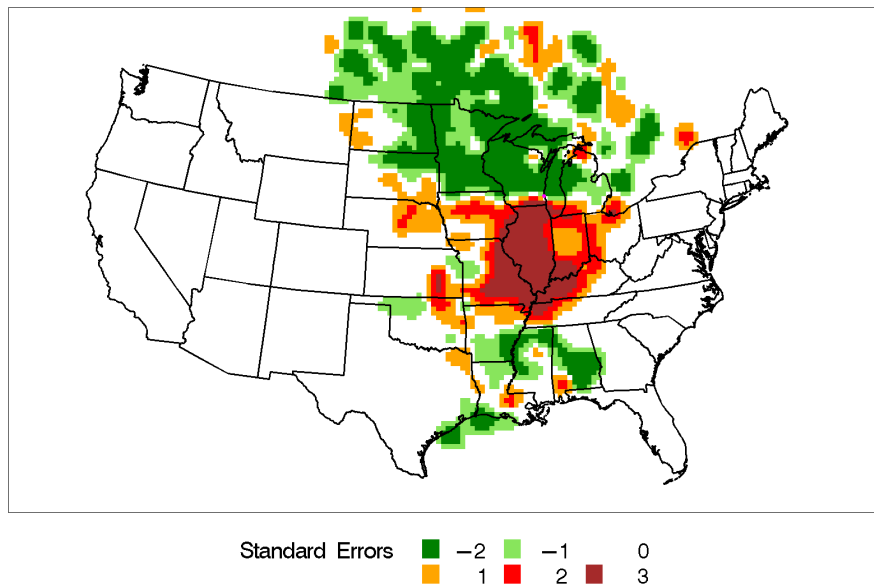
Milwaukee, WI, Source 8 Incremental Probability for High Source Strength
