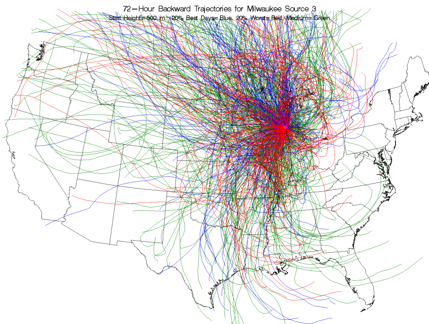
Figure I-17 Back Trajectories Color Coded by Source Strength Category for Milwaukee, Wisconsin, Source 3 - Crustal.
