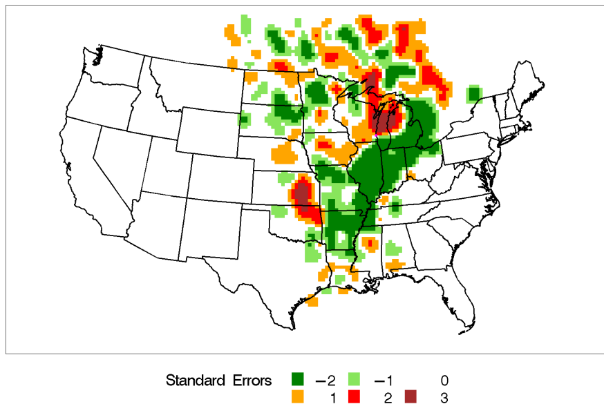
Figure I-22 Incremental Probability Contour Plot for Milwaukee, Wisconsin, Source 4 - Chlorine Sources.
