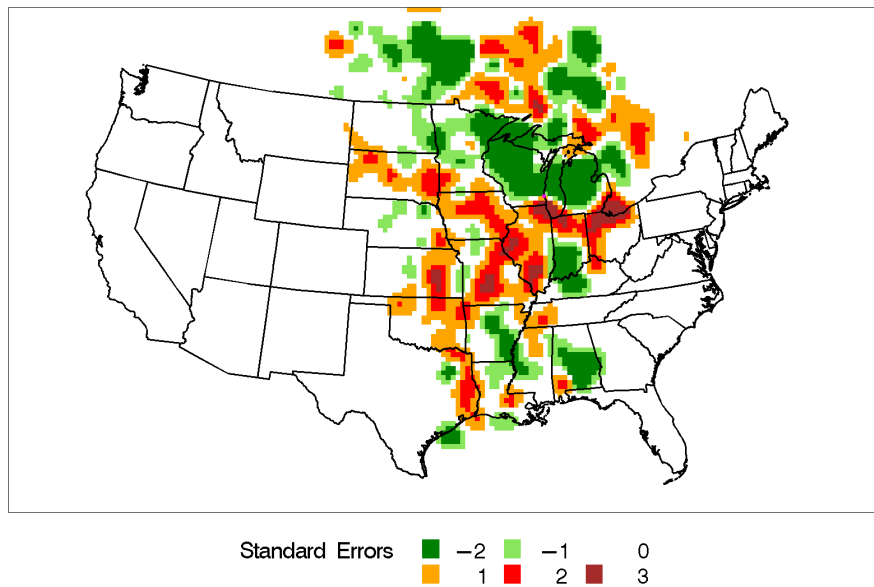
Figure I-16 Incremental Probability Contour Plot for Milwaukee, Wisconsin, Source 3 - Crustal.
