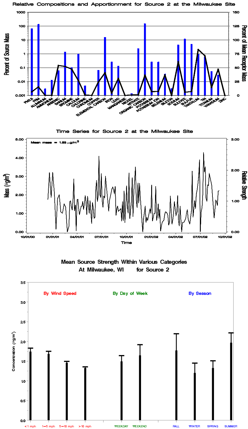
Figure I-7. Profile Plot (Top), Time Series Plot (Middle), and Bar Charts of the Source Strength Averaged by Wind Speed, Day of Week, and Season (Bottom) for Milwaukee, Wisconsin, Source 2 - Mobile Sources.
