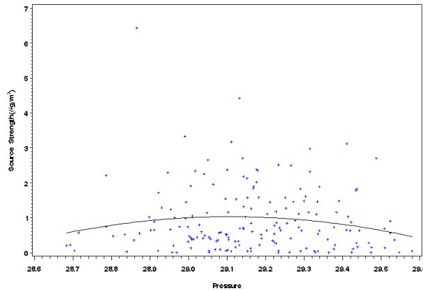
Figure I-48 Scatter Plot of Source Strength Versus Mean Daily Temperature (Rows 1 and 2) and Pressure (bottom) for Milwaukee, Wisconsin, Source 8 - Industrial Diesel and Sulfate Mix.
