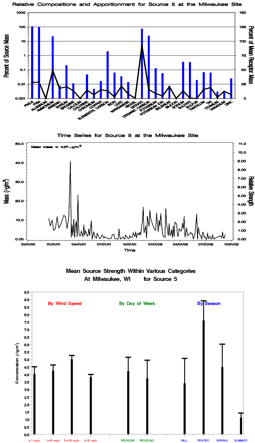
Figure I-25 Profile Plot (Top), Time Series Plot (Middle), and Bar Charts of the Source Strength Averaged by Wind Speed, Day of Week, and Season (Bottom) for Milwaukee, Wisconsin, Source 5 - Ammonium Nitrate.
