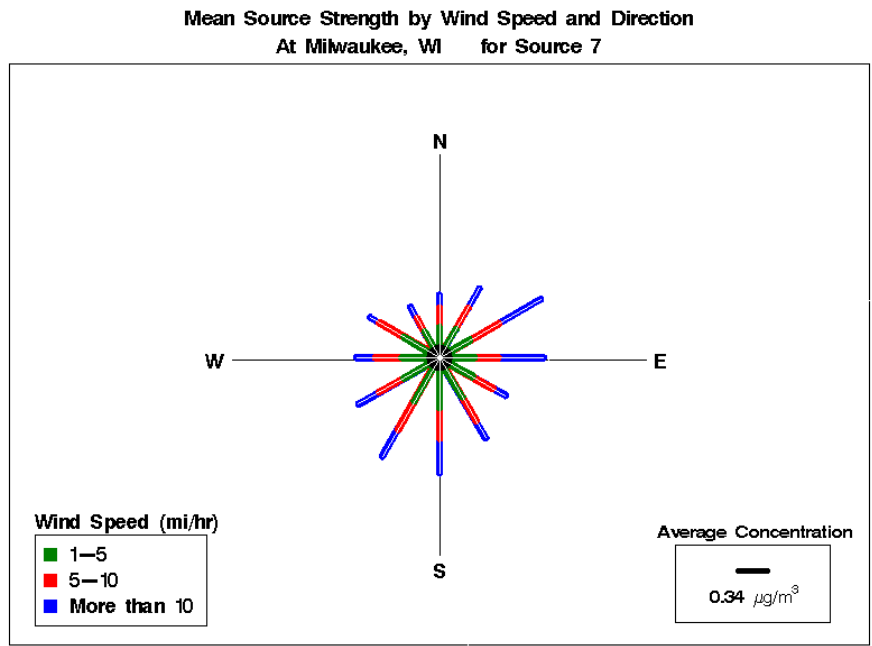
Figure I-38 Pollution Rose for Milwaukee, Wisconsin, Source 7 - Vegetative Burning and Fireworks.
