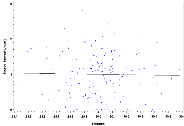
Figure E-18. Scatter Plot of Source Strength Versus Mean Daily Temperature (Rows 1 and 2) and Pressure (bottom) for Bronx, New York, Source 3 - Marine and Industrial Salts.
