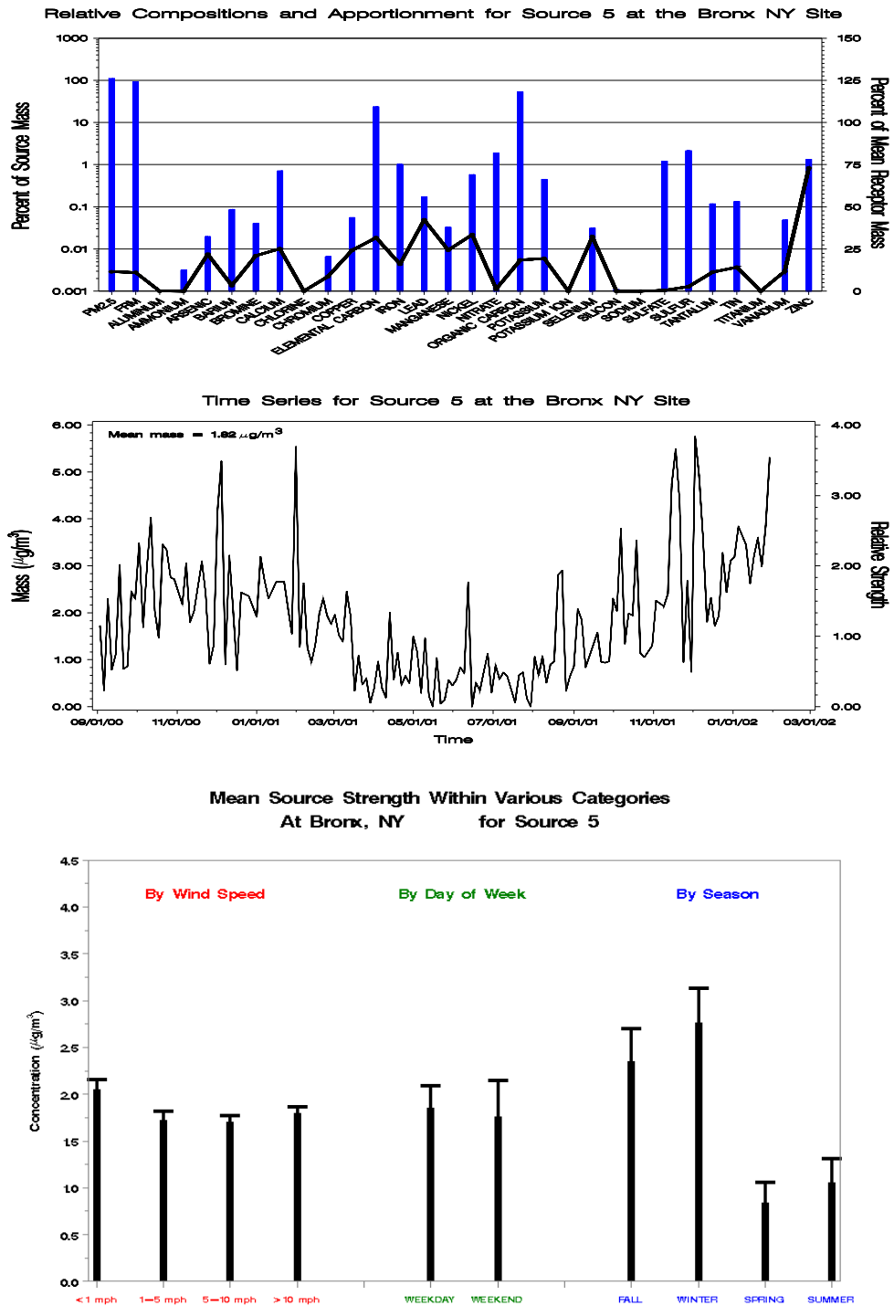
Figure E-25. Profile Plot (Top), Time Series Plot (Center), and Bar Charts of the Source Strength Averaged by Wind Speed, Day of Week, and Season (Bottom) for Bronx, New York, Source 5 - Industrial.
