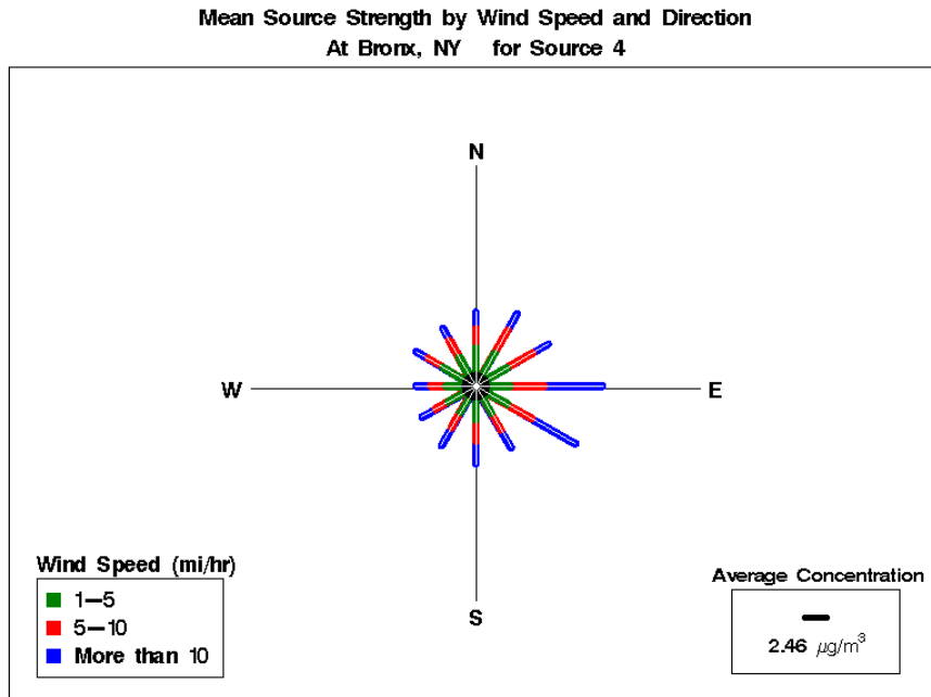
Figure E-20. Pollution Rose for Bronx, New York, Source 4 - Mobile Sources with Tire Wear.
