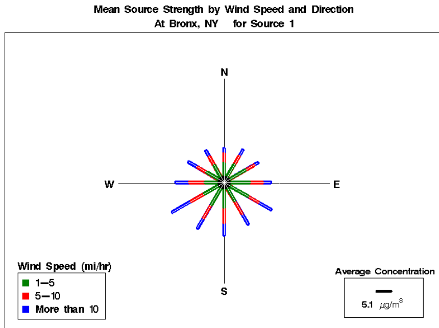
Figure E-2. Pollution Rose for Bronx, New York, Source 1 - Coal Combustion.
