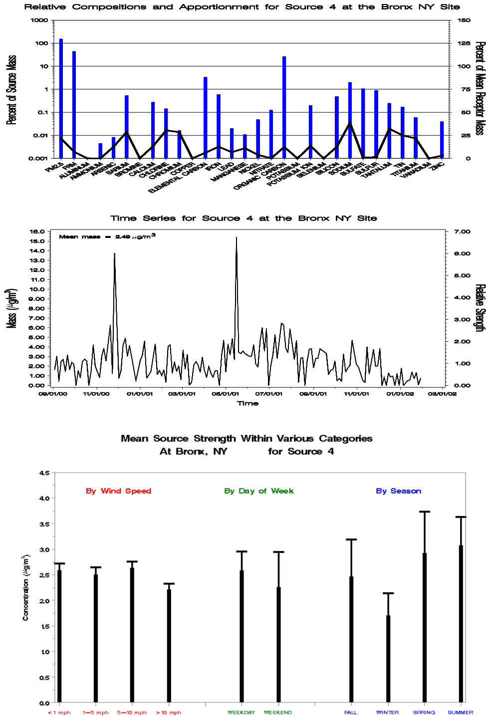
Figure E-19. Profile Plot (Top), Time Series Plot (Center), and Bar Charts of the Source Strength Averaged by Wind Speed, Day of Week, and Season (Bottom) for Bronx, New York, Source 4 - Mobile Sources with Tire Wear.
