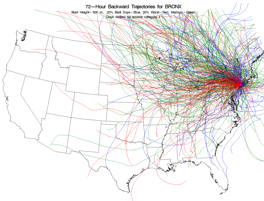
Figure E-41. Back Trajectories Color Coded by Source Strength Category for Bronx, New York, Source 7 - Crustal.
