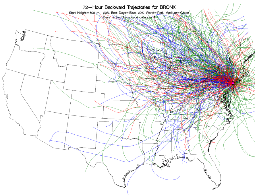
Figure E-23. Back Trajectories Color Coded by Source Strength Category for Bronx, New York, Source 4 - Mobile Sources with Tire Wear.
