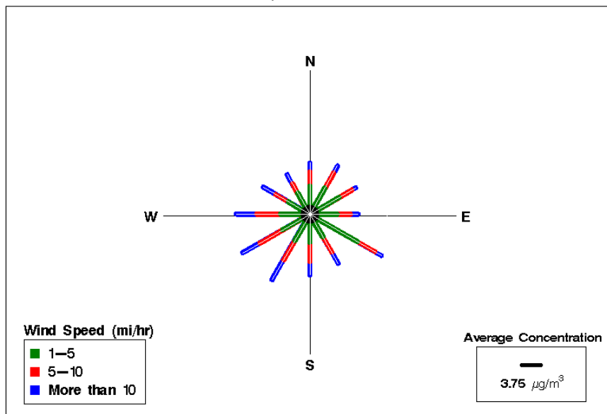
Mean Source Strength by Wind Speed and Direction At Bronx, NY for Source 6
