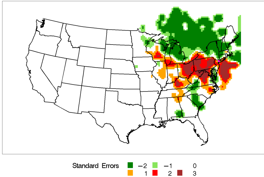
Figure E-4. Incremental Probability Contour Plot for Bronx, New York, Source 1 - Coal Combustion.
