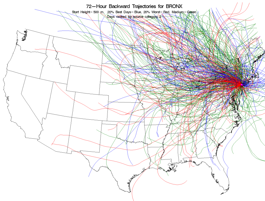
Figure E-11. Back Trajectories Color Coded by Source Strength Category for Bronx, New York, Source 2 - Oil Combustion.
