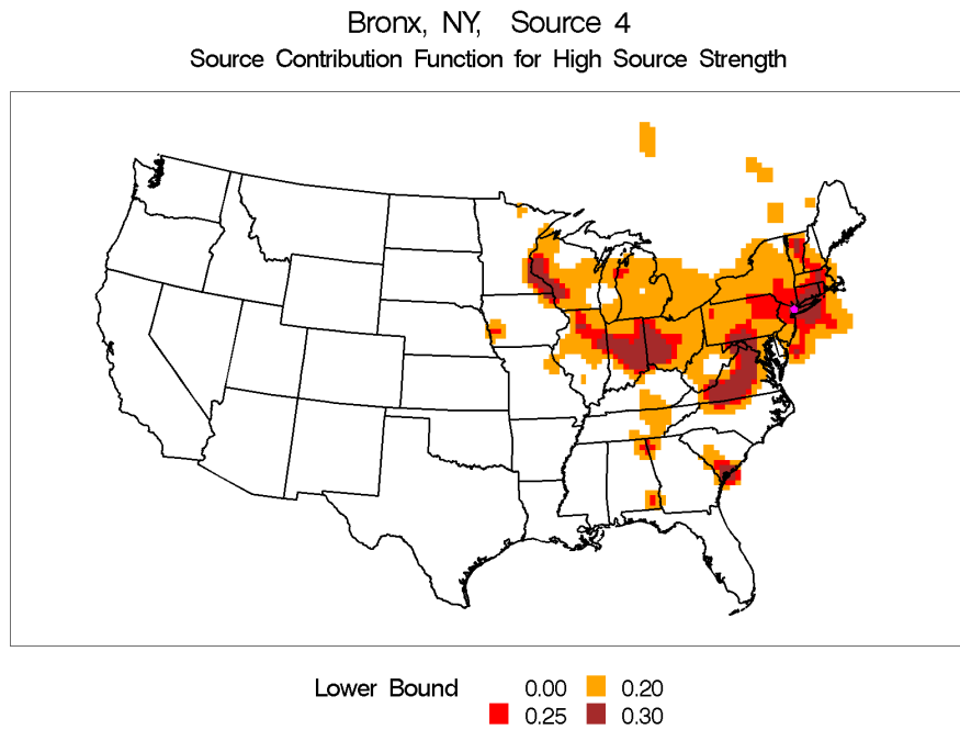
Figure E-21. Source Contribution Contour Plot for Bronx, New York, Source 4 - Mobile Sources with Tire Wear.
