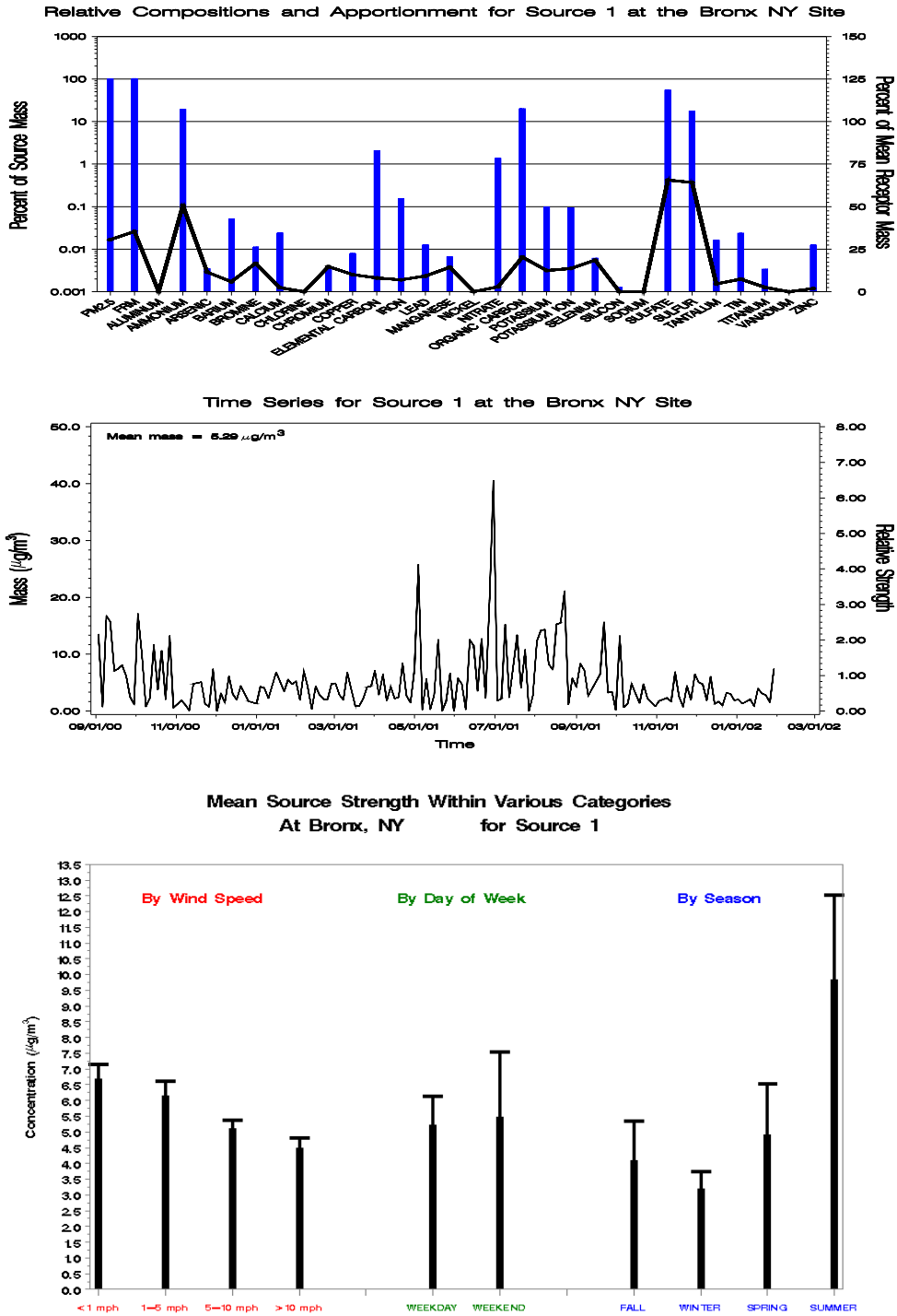
Figure E-1. Profile Plot (Top), Time Series Plot (Center), and Bar Charts of the Source Strength Averaged by Wind Speed, Day of Week, and Season (Bottom) for Bronx, New York, Source 1 - Coal Combustion.
