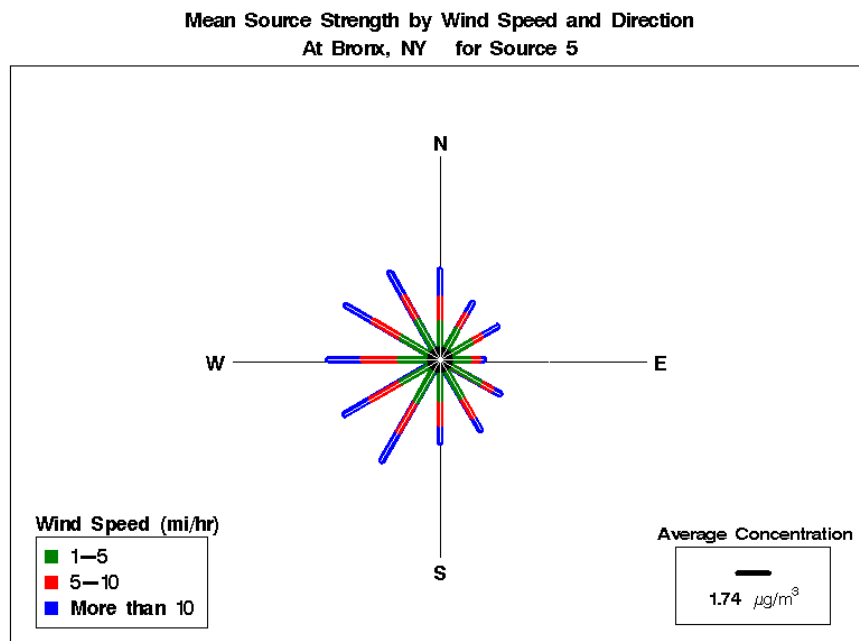
Figure E-26. Pollution Rose for Bronx, New York, Source 5 - Industrial.
