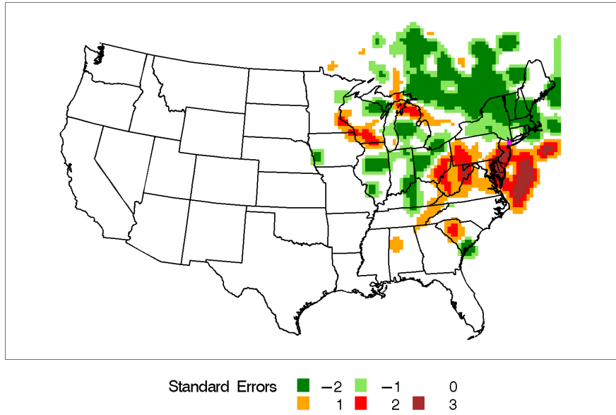
Figure E-16. Incremental Probability Contour Plot for Bronx, New York, Source 3 - Marine and Industrial Salts.
