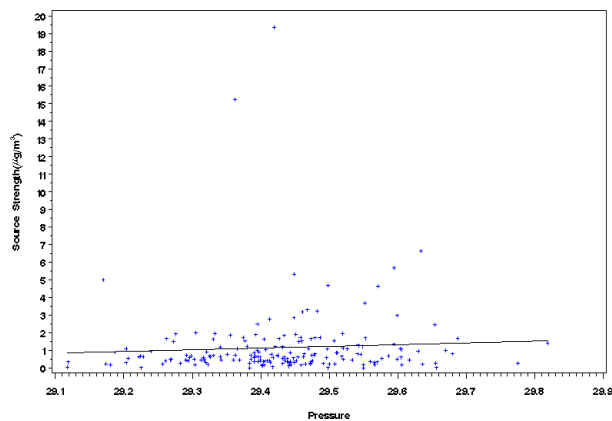
Figure E-24. Scatter Plot of Source Strength Versus Mean Daily Temperature (Rows 1 and 2) and Pressure (bottom) for Bronx, New York, Source 4 - Mobile Sources with Tire Wear.
