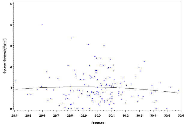
Figure E-12. Scatter Plot of Source Strength Versus Mean Daily Temperature (Rows 1 and 2) and Pressure (bottom) for Bronx, New York, Source 2 - Oil Combustion.
