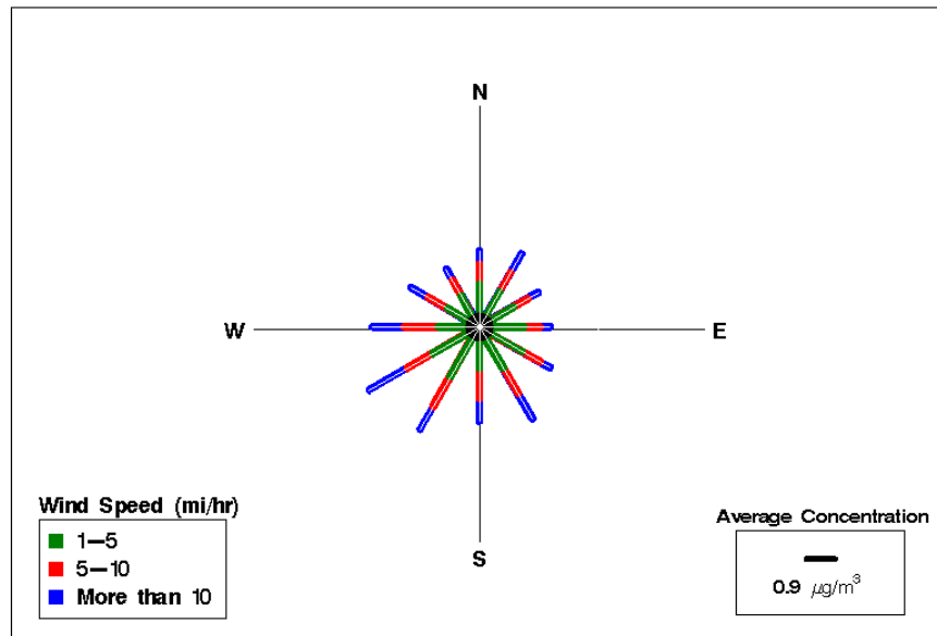
Mean Source Strength by Wind Speed and Direction At Bronx, NY for Source 7
