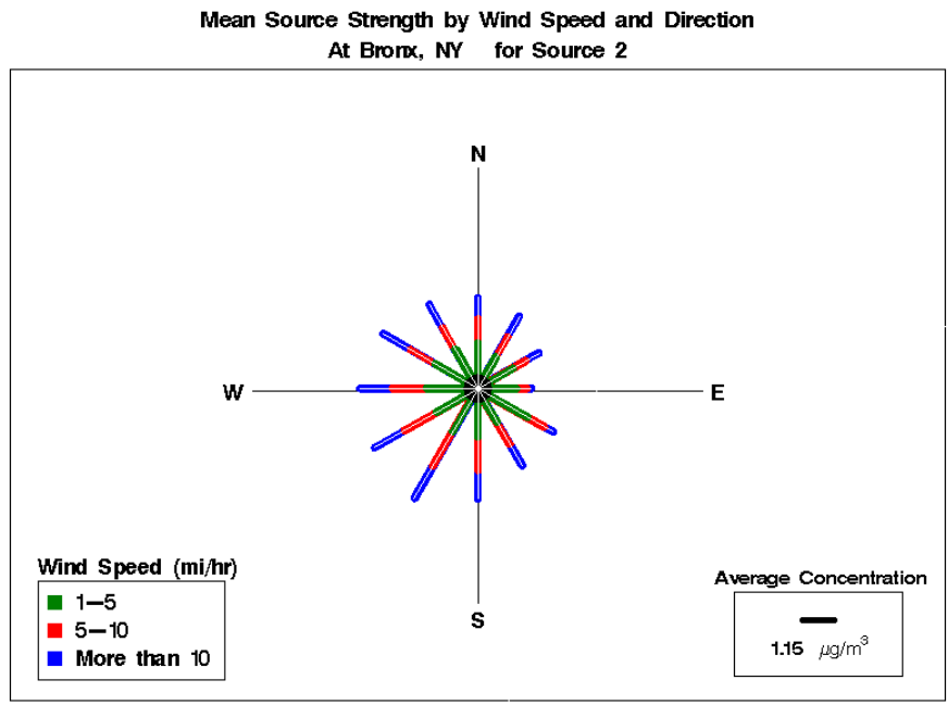
Figure E-8. Pollution Rose for Bronx, New York, Source 2 - Oil Combustion.
