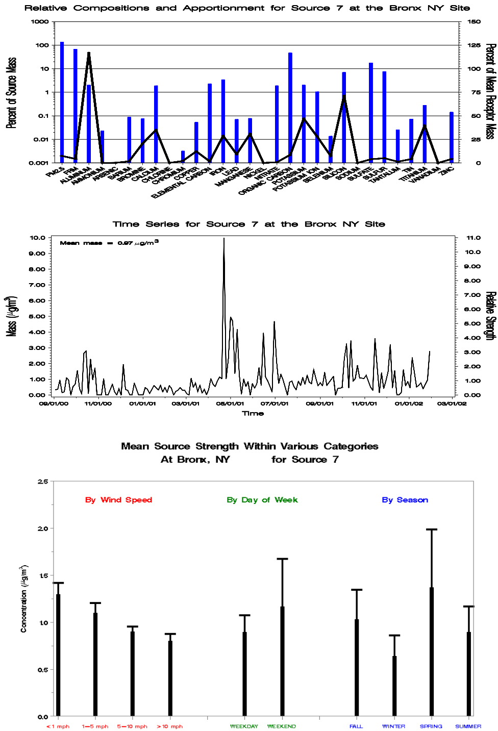
Figure E-37. Profile Plot (Top), Time Series Plot (Center), and Bar Charts of the Source Strength Averaged by Wind Speed, Day of Week, and Season (Bottom) for Bronx, New York, Source 7 - Crustal.
