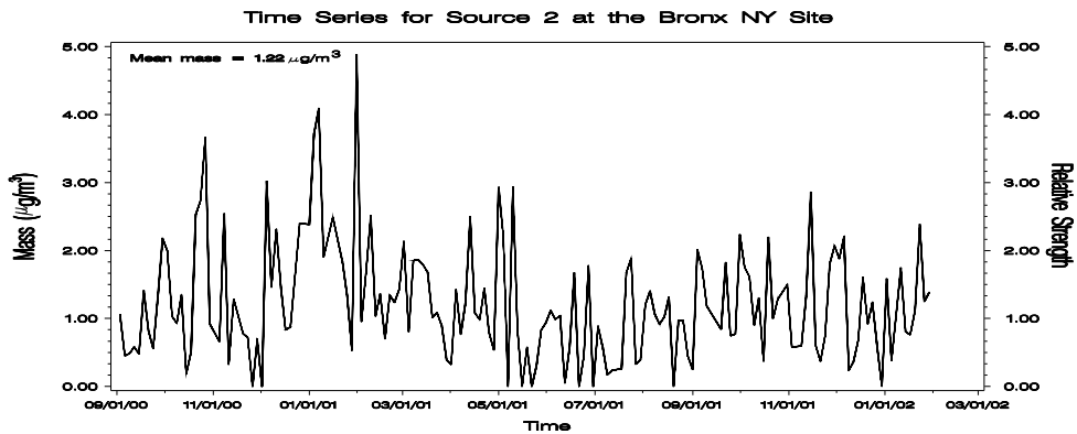
Mean Source Strength Within Various Categories At Bronx, NY for Source 2
