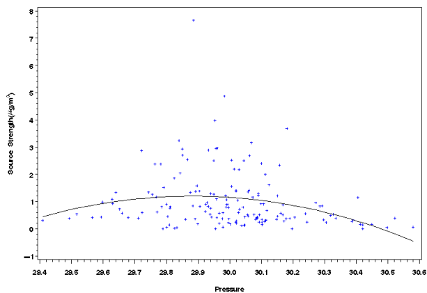
Figure E-6. Scatter Plot of Source Strength Versus Mean Daily Temperature (Rows 1 and 2) and Pressure (bottom) for Bronx, New York, Source 1 - Coal Combustion.
