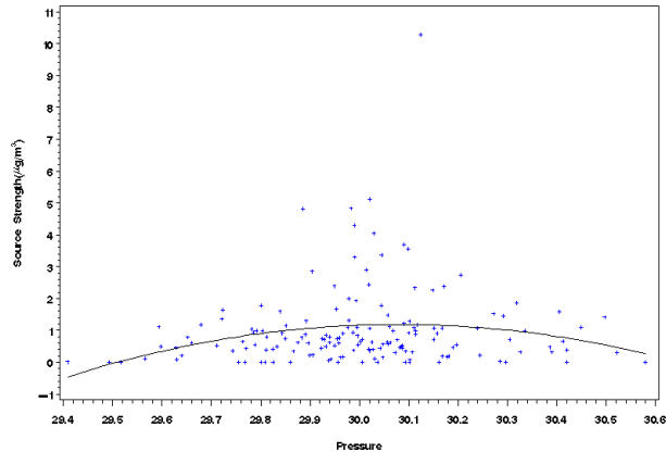
Figure E-42. Scatter Plot of Source Strength Versus Mean Daily Temperature (Rows 1 and 2) and Pressure (bottom) for Bronx, New York, Source 7 - Crustal.
