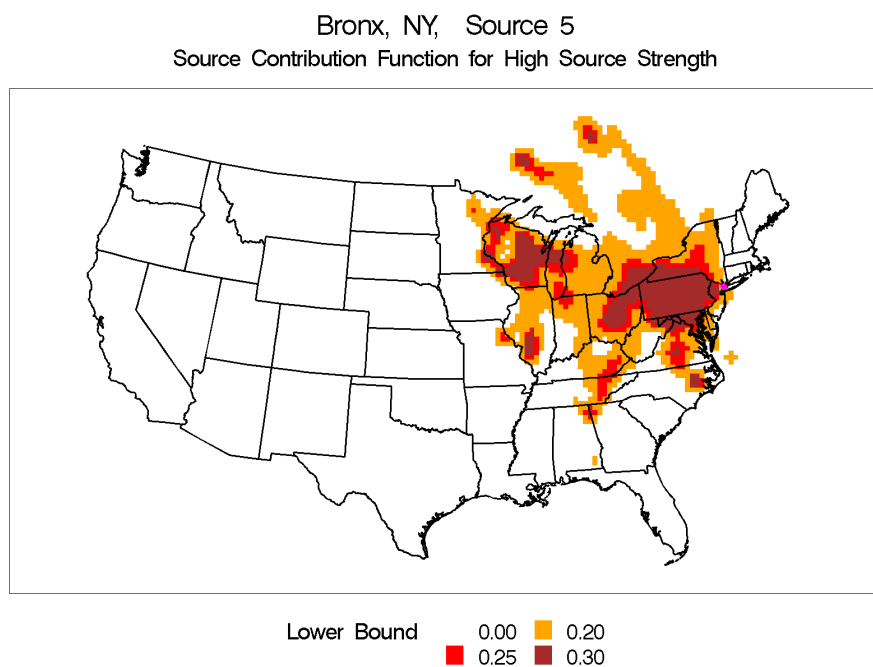
Figure E-27. Source Contribution Contour Plot for Bronx, New York, Source 5 - Industrial.
