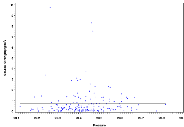
Figure E-30. Scatter Plot of Source Strength Versus Mean Daily Temperature (Rows 1 and 2) and Pressure (bottom) for Bronx, New York, Source 5 - Industrial.
