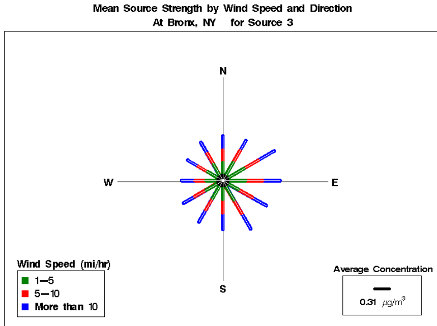
Figure E-14. Pollution Rose for Bronx, New York, Source 3 - Marine and Industrial Salts.
