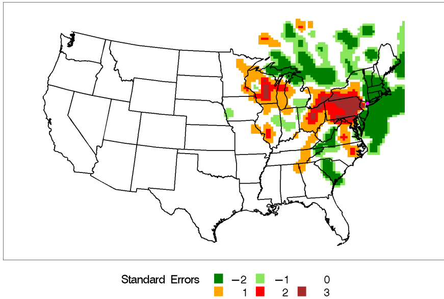
Figure E-28. Incremental Probability Contour Plot for Bronx, New York, Source 5 - Industrial.
