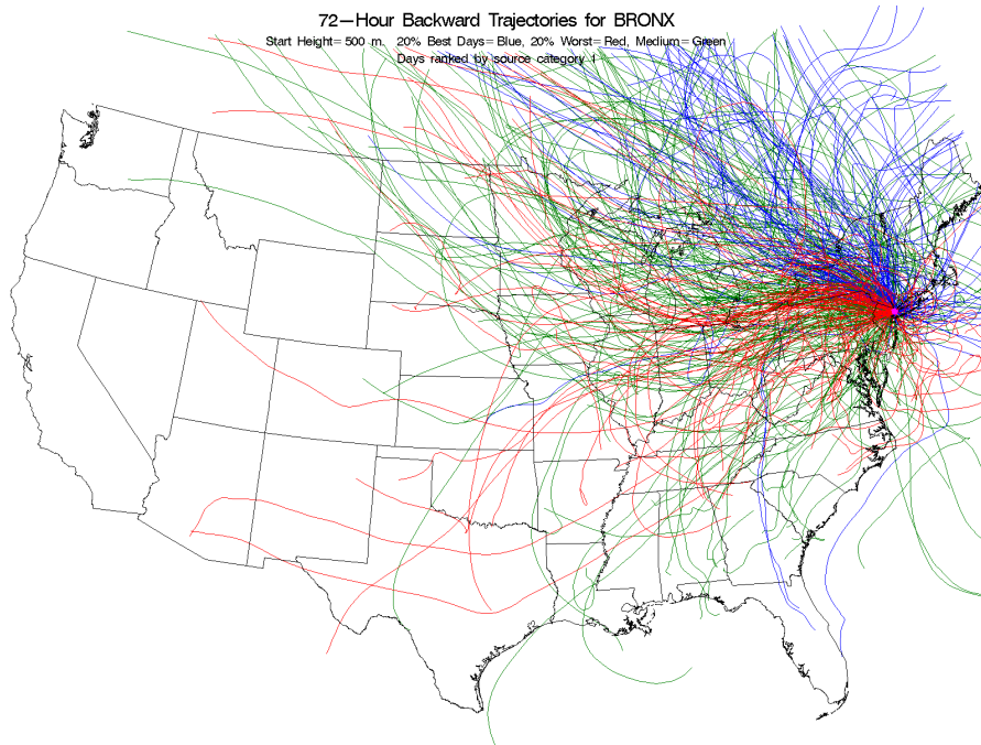
Figure E-5. Back Trajectories Color Coded by Source Strength Category for Bronx, New York, Source 1 - Coal Combustion.
