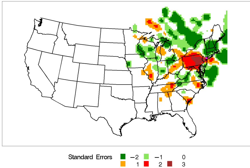
Figure E-10. Incremental Probability Contour Plot for Bronx, New York, Source 2 - Oil Combustion.
