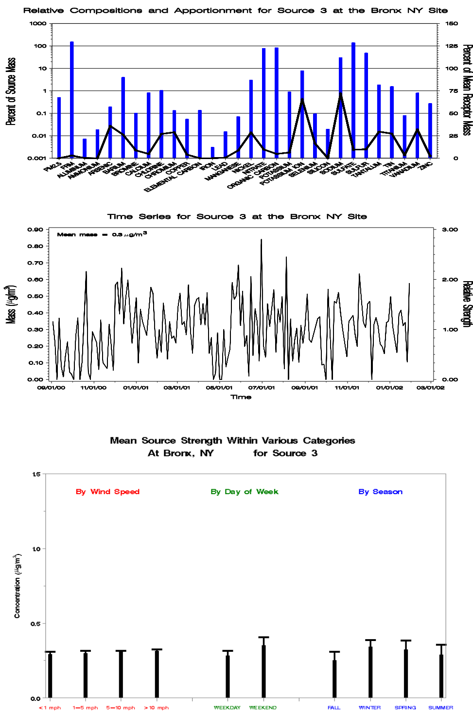
Figure E-13. Profile Plot (Top), Time Series Plot (Center), and Bar Charts of the Source Strength Averaged by Wind Speed, Day of Week, and Season (Bottom) for Bronx, New York, Source 3 - Marine and Industrial Salts.
