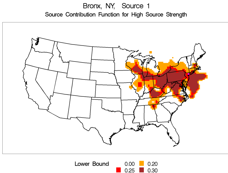
Figure E-3. Source Contribution Contour Plot for Bronx, New York, Source 1 - Coal Combustion.
