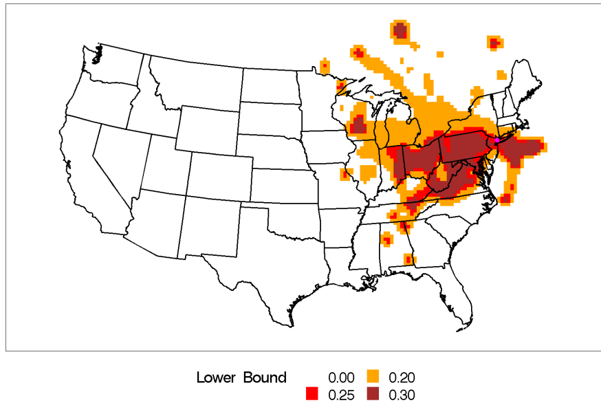
Bronx, NY, Source 7 Source Contribution Function for High Source Strength
