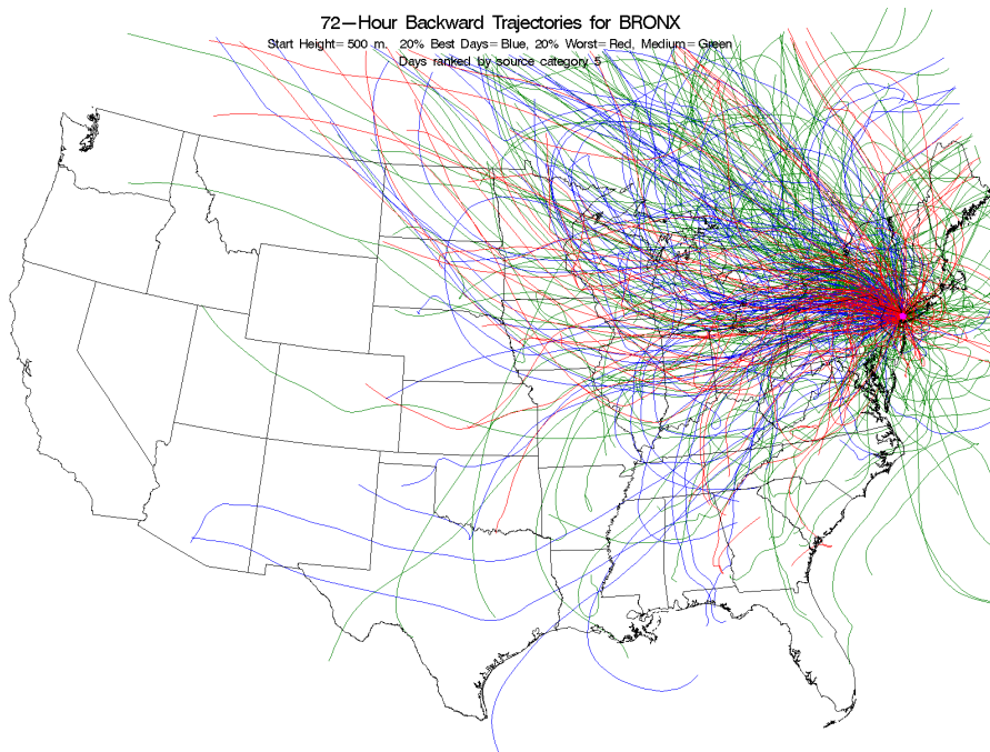
Figure E-29. Back Trajectories Color Coded by Source Strength Category for Bronx, New York, Source 5 - Industrial.
