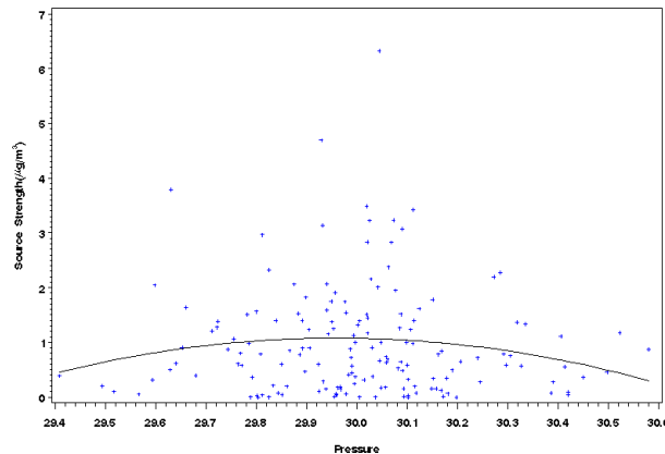
Figure E-36. Scatter Plot of Source Strength Versus Mean Daily Temperature (Rows 1 and 2) and Pressure (bottom) for Bronx, New York, Source 6 - Ammonium Nitrate.
