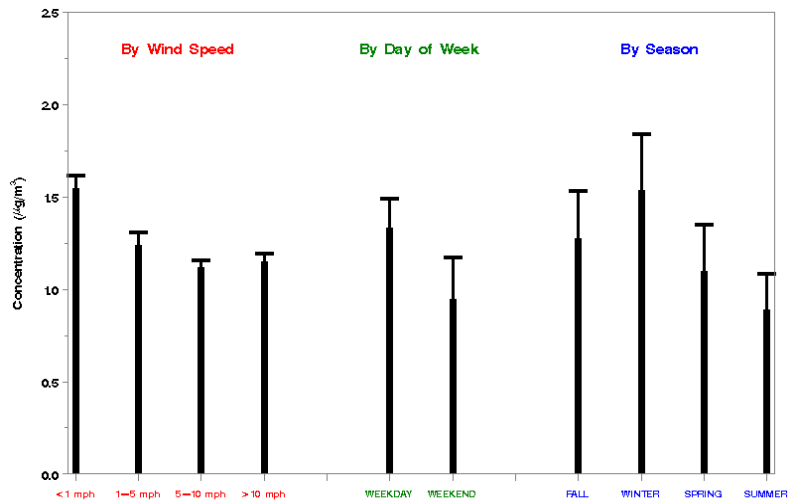
Figure E-7. Profile Plot (Top), Time Series Plot (Center), and Bar Charts of the Source Strength Averaged by Wind Speed, Day of Week, and Season (Bottom) for Bronx, New York, Source 2 - Oil Combustion.
