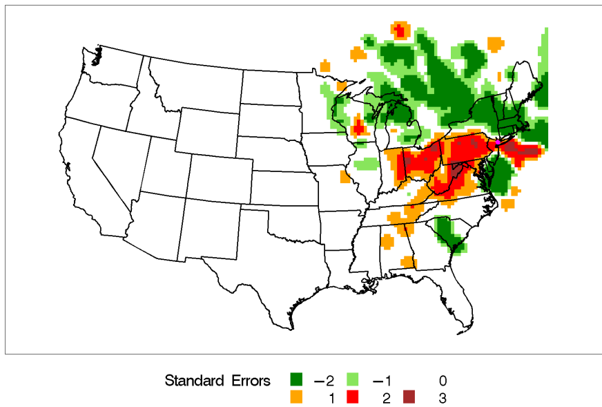
Figure E-40. Incremental Probability Contour Plot for Bronx, New York, Source 7 - Crustal.
