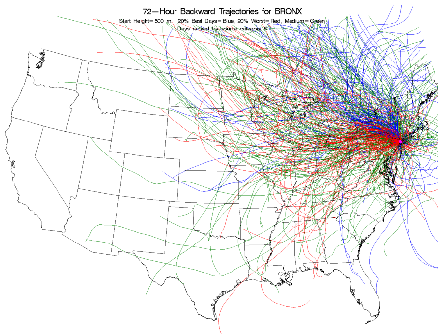
Figure E-35. Back Trajectories Color Coded by Source Strength Category for Bronx, New York, Source 6 - Ammonium Nitrate.
