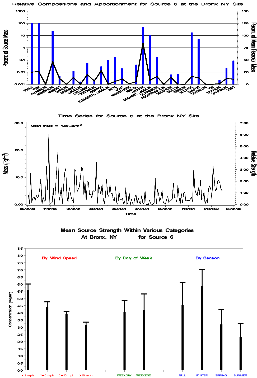
Figure E-31. Profile Plot (Top), Time Series Plot (Center), and Bar Charts of the Source Strength Averaged by Wind Speed, Day of Week, and Season (Bottom) for Bronx, New York, Source 6 - Ammonium Nitrate.
