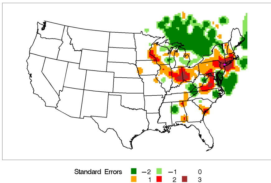
Figure E-22. Incremental Probability Contour Plot for Bronx, New York, Source 4 - Mobile Sources with Tire Wear.
