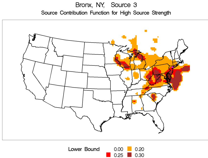
Figure E-15. Source Contribution Contour Plot for Bronx, New York, Source 3 - Marine and Industrial Salts.
