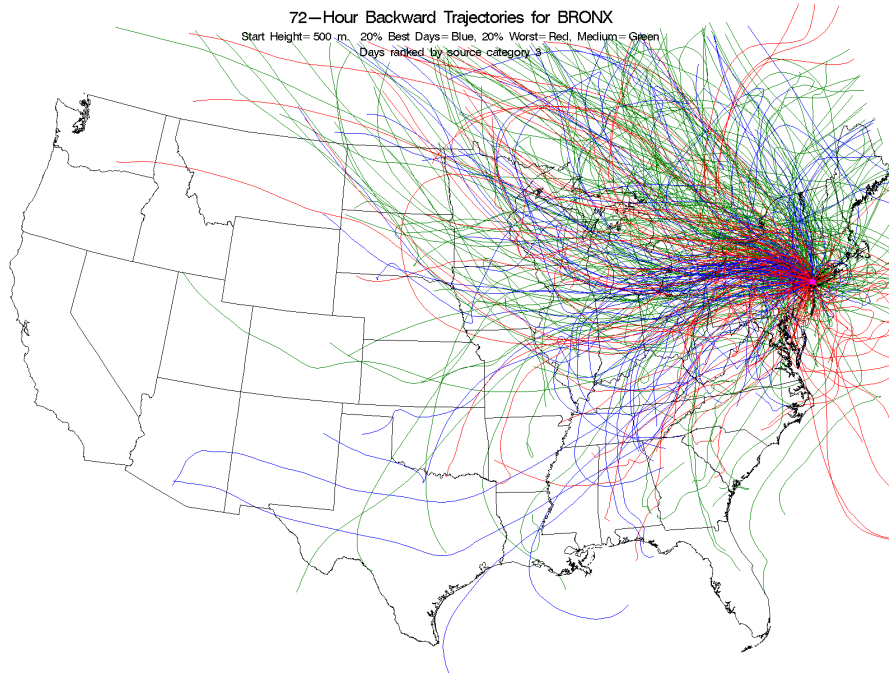
Figure E-17. Back Trajectories Color Coded by Source Strength Category for Bronx, New York, Source 3 - Marine and Industrial Salts.
