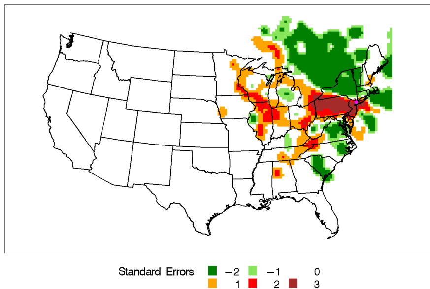
Figure E-34. Incremental Probability Contour Plot for Bronx, New York, Source 6 - Ammonium Nitrate.
