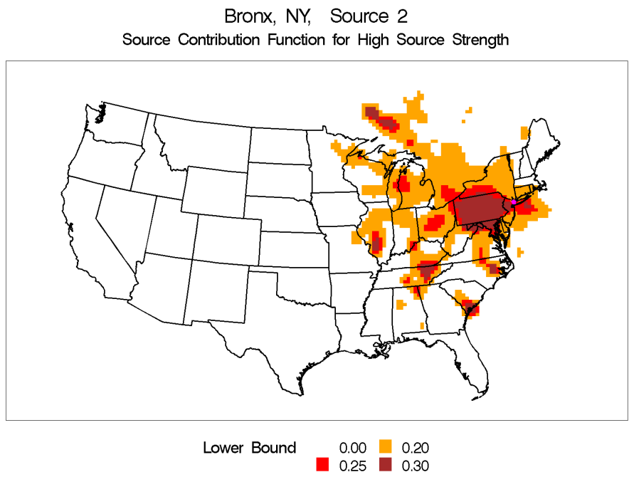
Figure E-9. Source Contribution Contour Plot for Bronx, New York, Source 2 - Oil Combustion.
