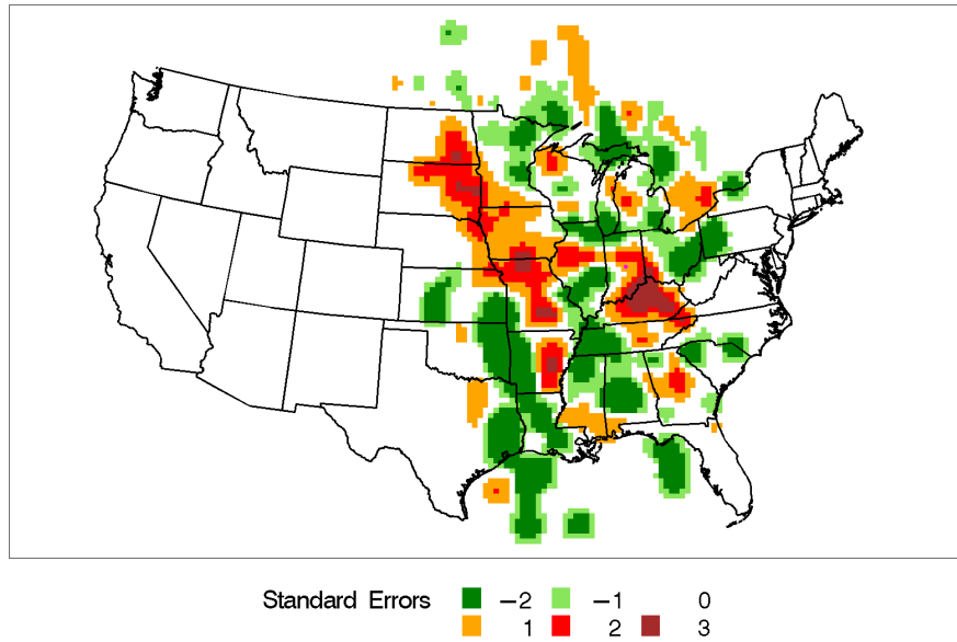
Figure H-16 Incremental Probability Contour Plot for Indianapolis, Indiana, Source 3 – Canadian Fires.
