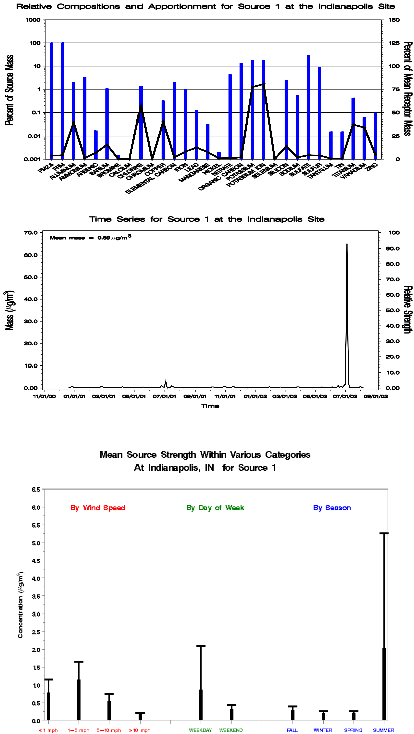
Figure H-1. Profile Plot (Top), Time Series Plot (Middle), and Bar Charts of the Source Strength Averaged by Wind Speed, Day of Week, and Season (Bottom) for Indianapolis, Indiana, Source 1 – Vegetative Burning and Fireworks.
