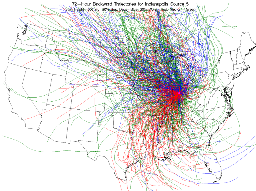
Figure H-29 Back Trajectories Color Coded by Source Strength Category for Indianapolis, Indiana, Source 5 – Crustal.
