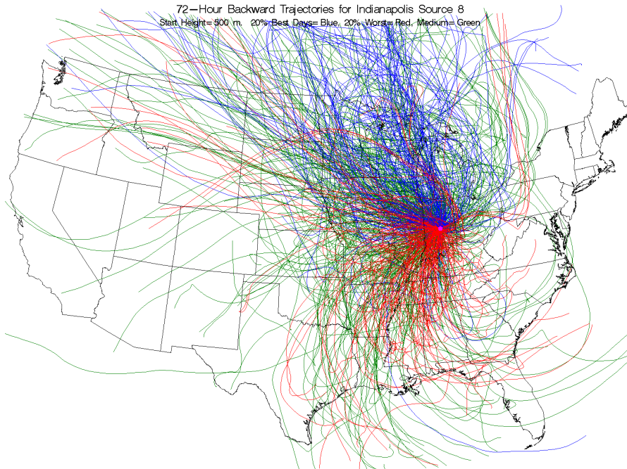
Figure H-47 Back Trajectories Color Coded by Source Strength Category for Indianapolis, Indiana, Source 8 – Coal Combustion 2 (Ni).
