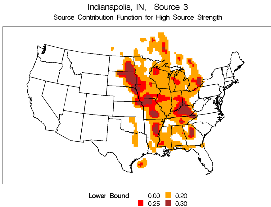
Figure H-15 Source Contribution Contour Plot for Indianapolis, Indiana, Source 3 – Canadian Fires.
