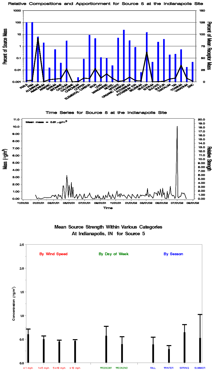
Figure H-25. Profile Plot (Top), Time Series Plot (Middle), and Bar Charts of the Source Strength Averaged by Wind Speed, Day of Week, and Season (Bottom) for Indianapolis, Indiana, Source 5 – Crustal.
