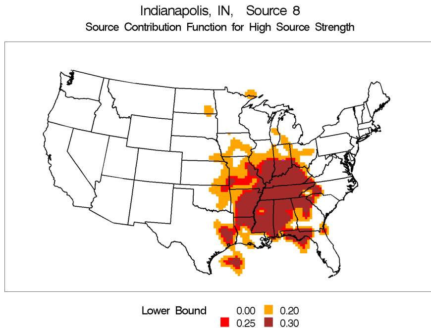
Figure H-45 Source Contribution Contour Plot for Indianapolis, Indiana, Source 8 – Coal Combustion 2 (Ni).
