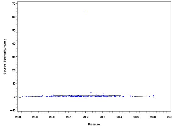
Figure H-6 Scatter Plot of Source Strength Versus Mean Daily Temperature (Rows 1 and 2) and Pressure (bottom) for Indianapolis, Indiana, Source 1 – Vegetative Burning and Fireworks.
