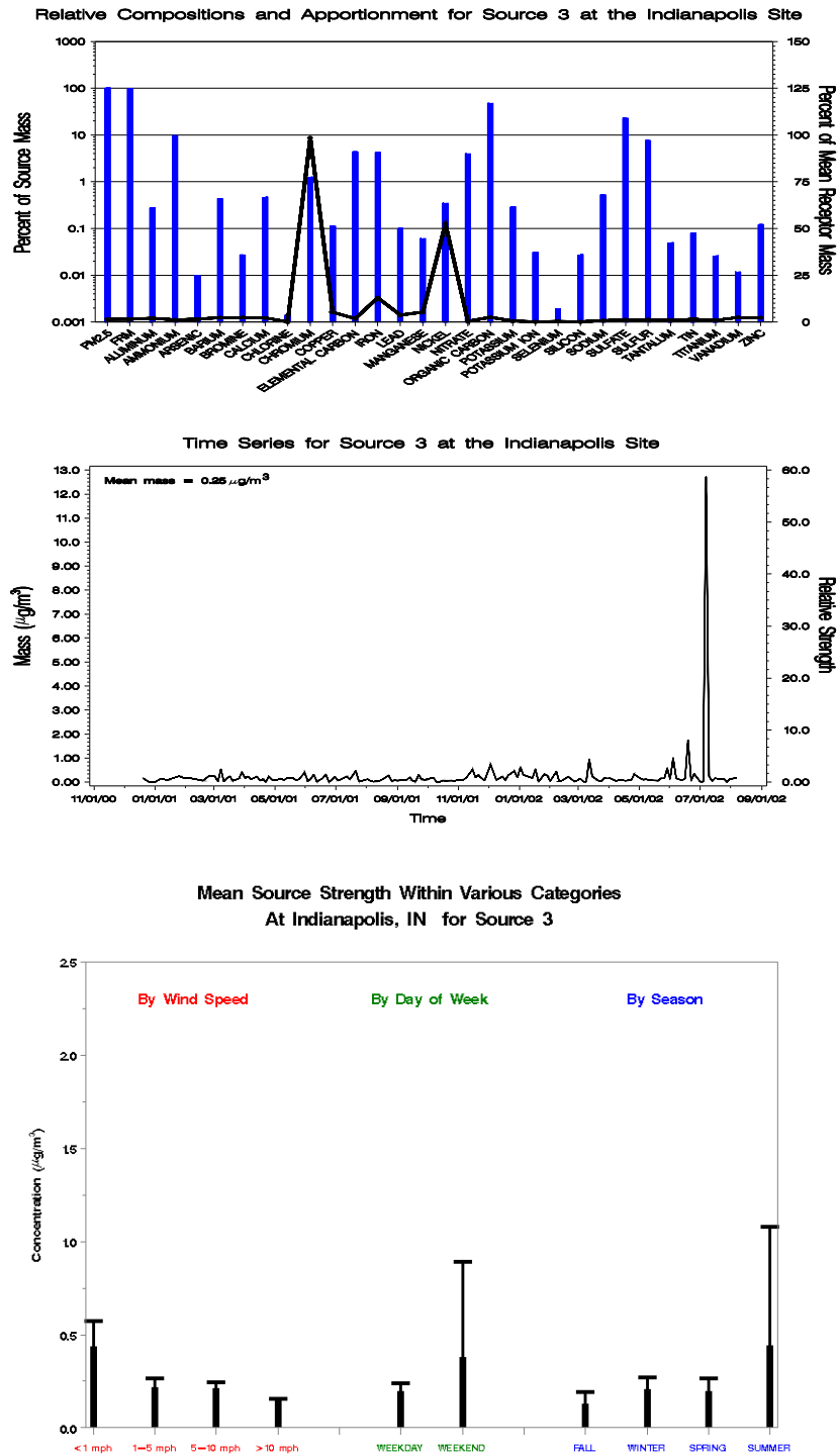
Figure H-13. Profile Plot (Top), Time Series Plot (Middle), and Bar Charts of the Source Strength Averaged by Wind Speed, Day of Week, and Season (Bottom) for Indianapolis, Indiana, Source 3 – Canadian Fires.
