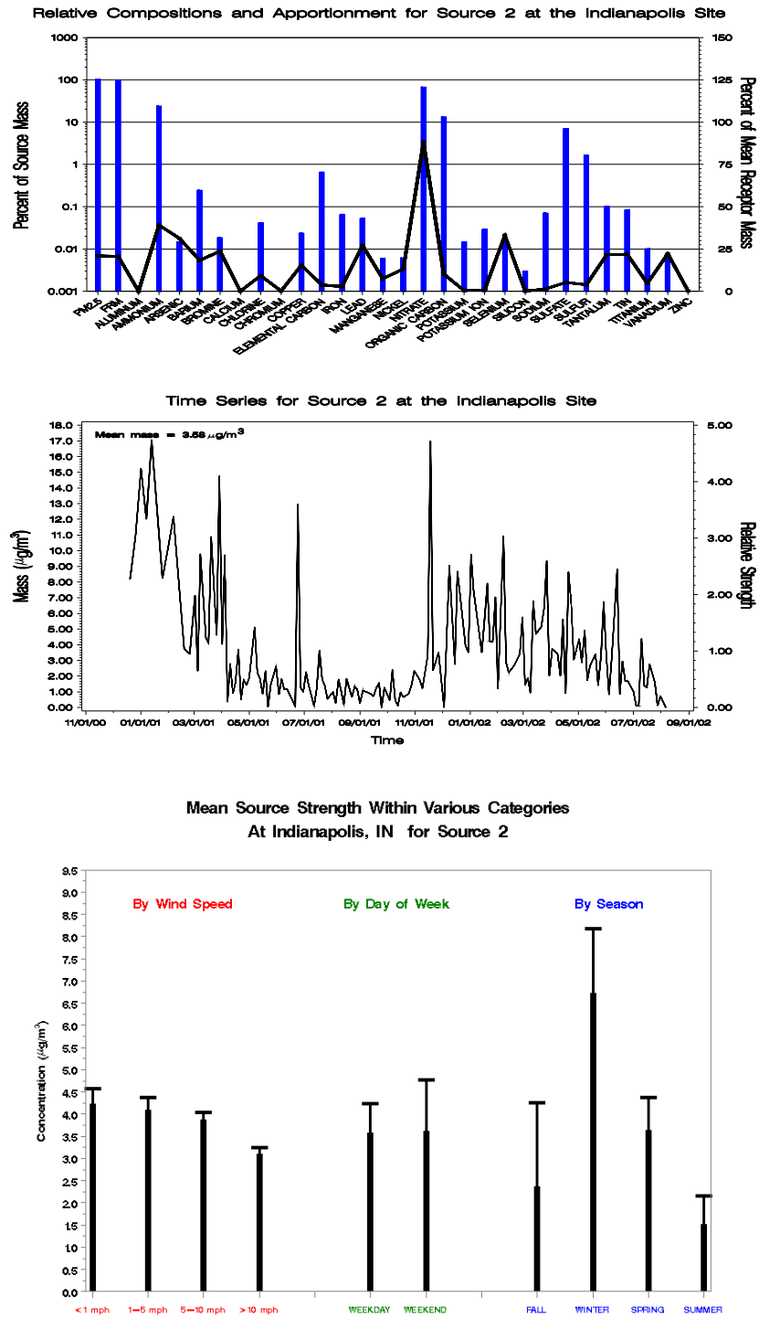
Figure H-7. Profile Plot (Top), Time Series Plot (Middle), and Bar Charts of the Source Strength Averaged by Wind Speed, Day of Week, and Season (Bottom) for Indianapolis, Indiana, Source 2 – Ammonium Nitrate.
