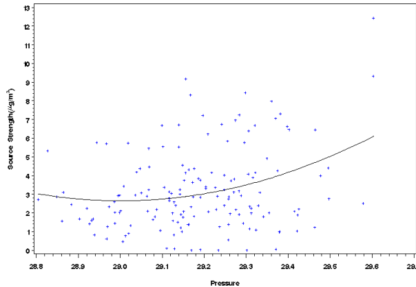
Figure H-36 Scatter Plot of Source Strength Versus Mean Daily Temperature (Rows 1 and 2) and Pressure (bottom) for Indianapolis, Indiana, Source 6 – Mobile Sources.
