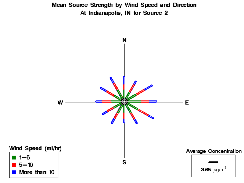
Figure H-8. Pollution Rose for Indianapolis, Indiana, Source 2 – Ammonium Nitrate.
