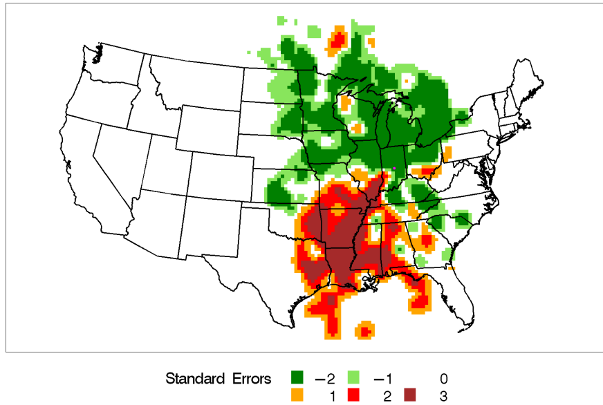
Figure H-28 Incremental Probability Contour Plot for Indianapolis, Indiana, Source 5 – Crustal.
