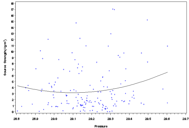
Figure H-12 Scatter Plot of Source Strength Versus Mean Daily Temperature (Rows 1 and 2) and Pressure (bottom) for Indianapolis, Indiana, Source 2 – Ammonium Nitrate.
