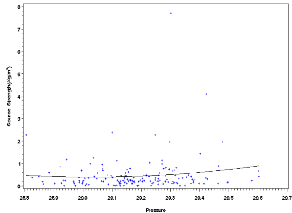
Figure H-24 Scatter Plot of Source Strength Versus Mean Daily Temperature (Rows 1 and 2) and Pressure (bottom) for Indianapolis, Indiana, Source 4 – Marine and Industrial Salts.
