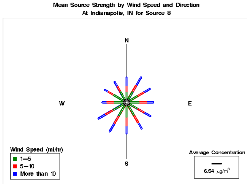
Figure H-44. Pollution Rose for Indianapolis, Indiana, Source 8 – Coal Combustion 2 (Ni).
