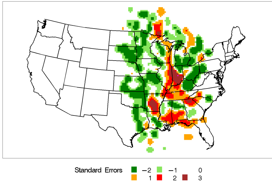
Figure H-4 Incremental Probability Contour Plot for Indianapolis, Indiana, Source 1 – Vegetative Burning and Fireworks.
