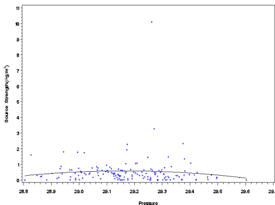
Figure H-30 Scatter Plot of Source Strength Versus Mean Daily Temperature (Rows 1 and 2) and Pressure (bottom) for Indianapolis, Indiana, Source 5 – Crustal.
