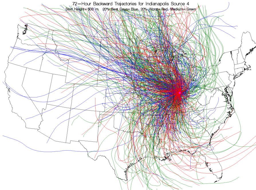
Figure H-23 Back Trajectories Color Coded by Source Strength Category for Indianapolis, Indiana, Source 4 – Marine and Industrial Salts.
