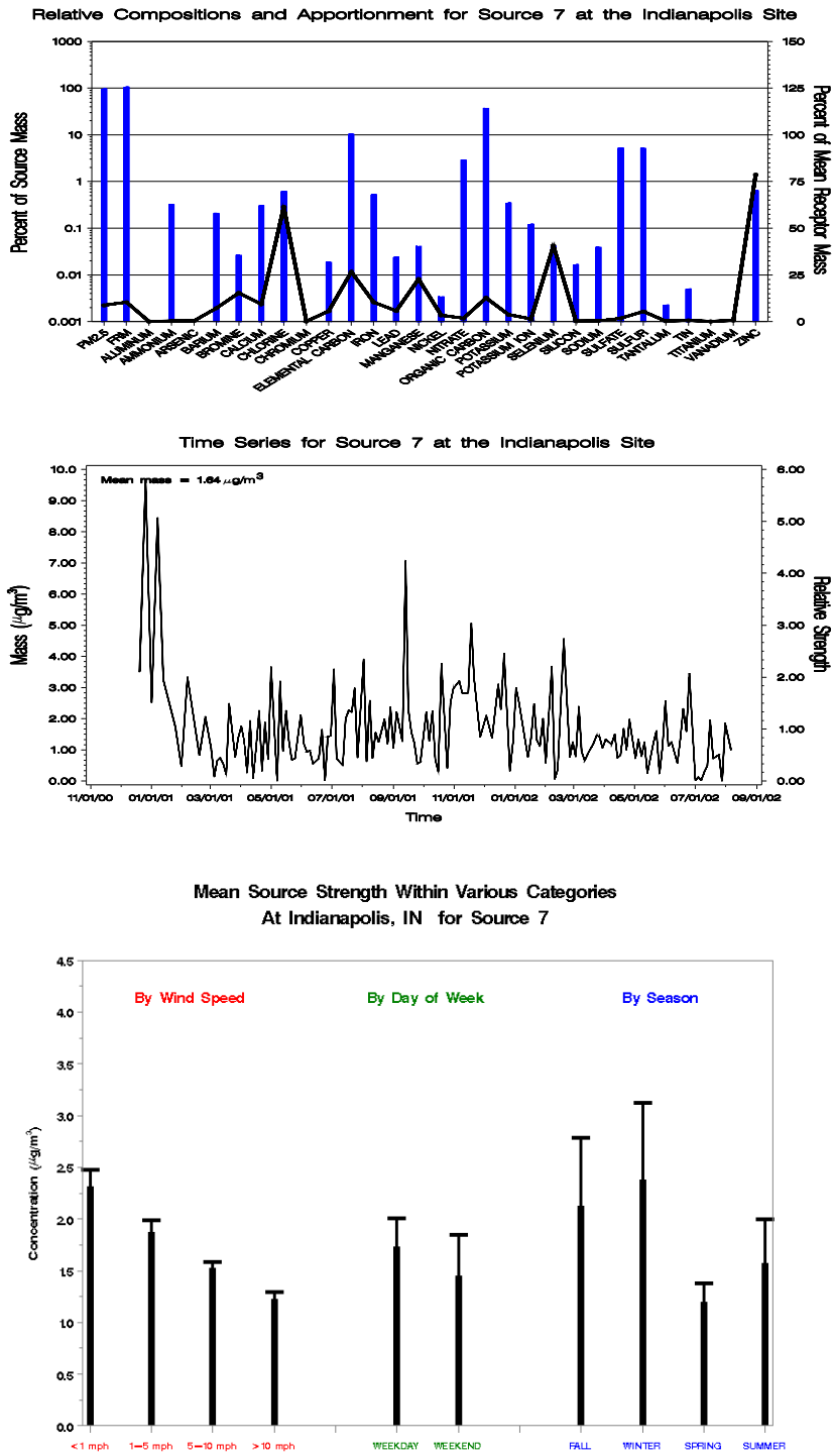
Figure H-37. Profile Plot (Top), Time Series Plot (Middle), and Bar Charts of the Source Strength Averaged by Wind Speed, Day of Week, and Season (Bottom) for Indianapolis, Indiana, Source 7 – Coal Combustion 1.
