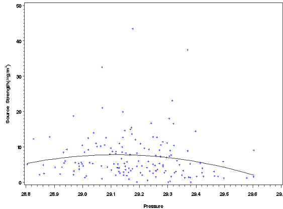
Figure H-48 Scatter Plot of Source Strength Versus Mean Daily Temperature (Rows 1 and 2) and Pressure (bottom) for Indianapolis, Indiana, Source 8 – Coal Combustion 2 (Ni).
