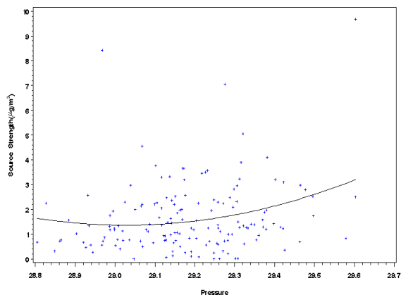
Figure H-42 Scatter Plot of Source Strength Versus Mean Daily Temperature (Rows 1 and 2) and Pressure (bottom) for Indianapolis, Indiana, Source 7 – Coal Combustion 1.
