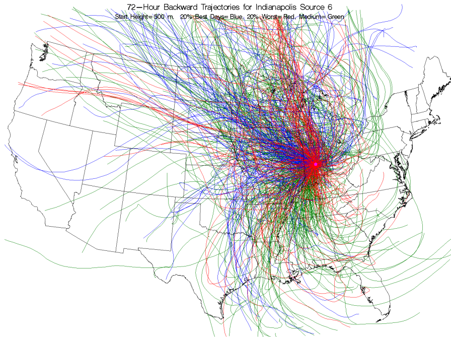
Figure H-35 Back Trajectories Color Coded by Source Strength Category for Indianapolis, Indiana, Source 6 – Mobile Sources.
