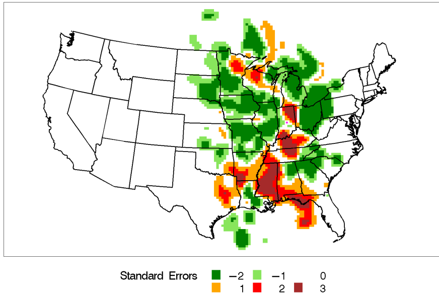
Figure H-22 Incremental Probability Contour Plot for Indianapolis, Indiana, Source 4 – Marine and Industrial Salts.
