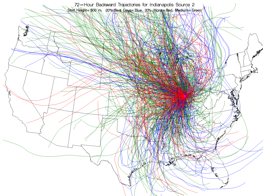
Figure H-11 Back Trajectories Color Coded by Source Strength Category for Indianapolis, Indiana, Source 2 – Ammonium Nitrate.
