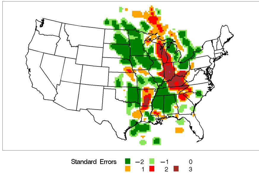
Indianapolis, IN, Source 6 Incremental Probability for High Source Strength
