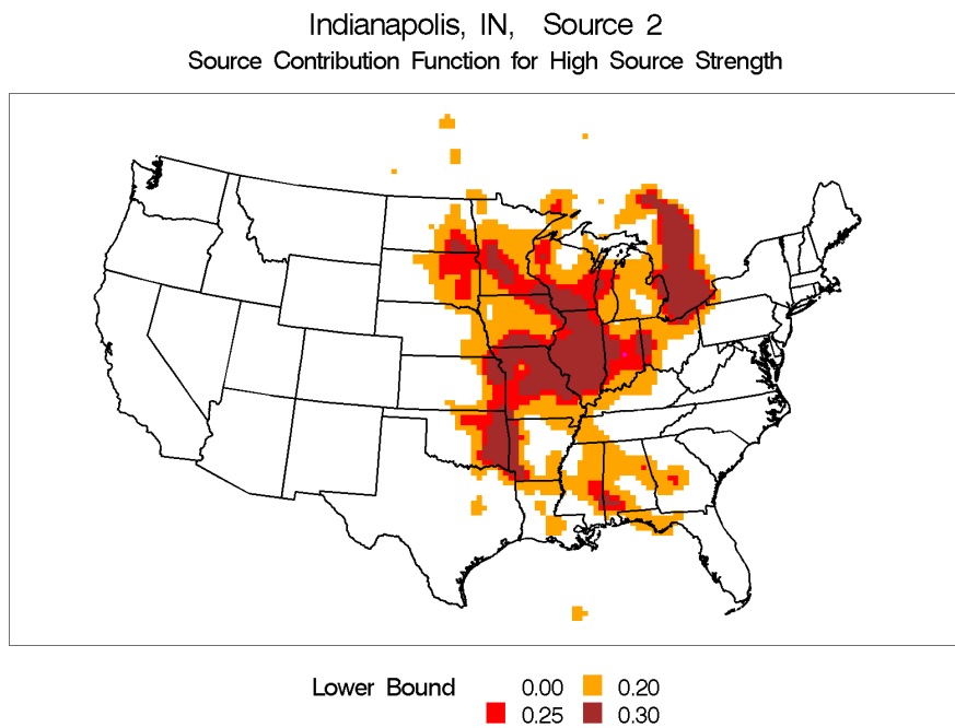
Figure H-9 Source Contribution Contour Plot for Indianapolis, Indiana, Source 2 – Ammonium Nitrate.
