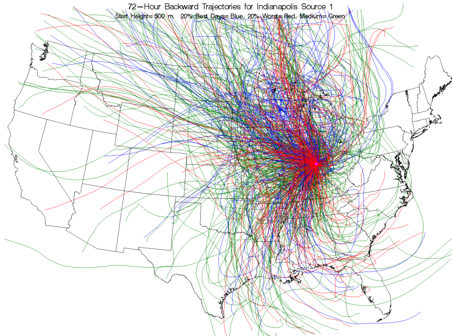
Figure H-5 Back Trajectories Color Coded by Source Strength Category for Indianapolis, Indiana, Source 1 – Vegetative Burning and Fireworks.
