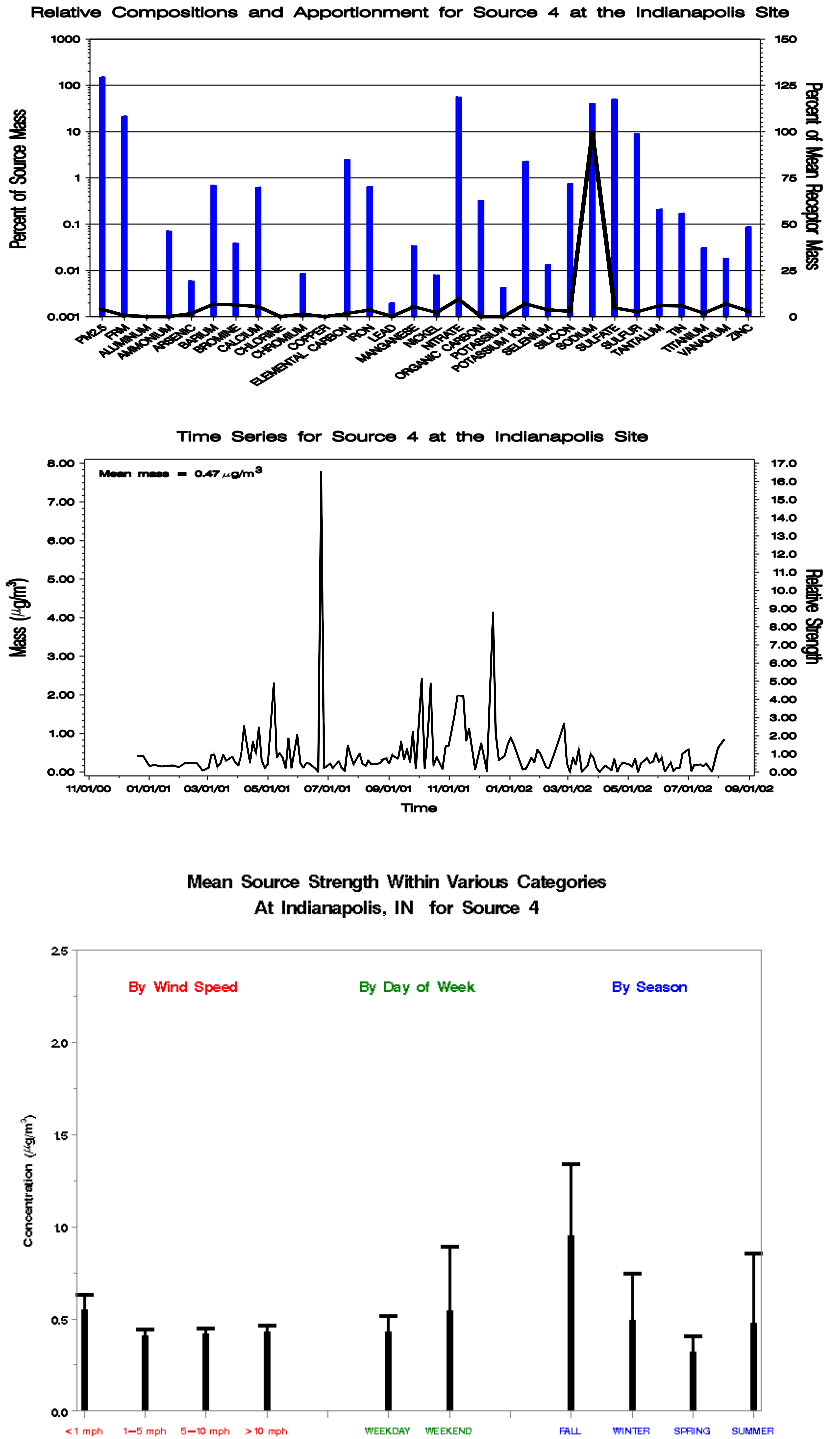
Figure H-19. Profile Plot (Top), Time Series Plot (Middle), and Bar Charts of the Source Strength Averaged by Wind Speed, Day of Week, and Season (Bottom) for Indianapolis, Indiana, Source 4 – Marine and Industrial Salts.
