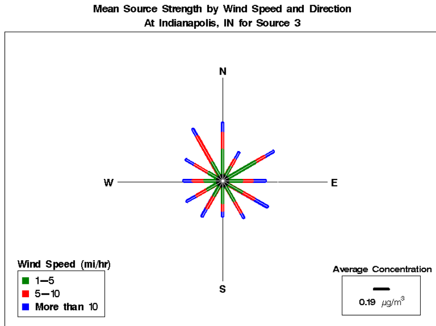
Figure H-14. Pollution Rose for Indianapolis, Indiana, Source 3 – Canadian Fires.
