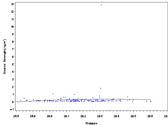
Figure H-18 Scatter Plot of Source Strength Versus Mean Daily Temperature (Rows 1 and 2) and Pressure (bottom) for Indianapolis, Indiana, Source 3 – Canadian Fires.
