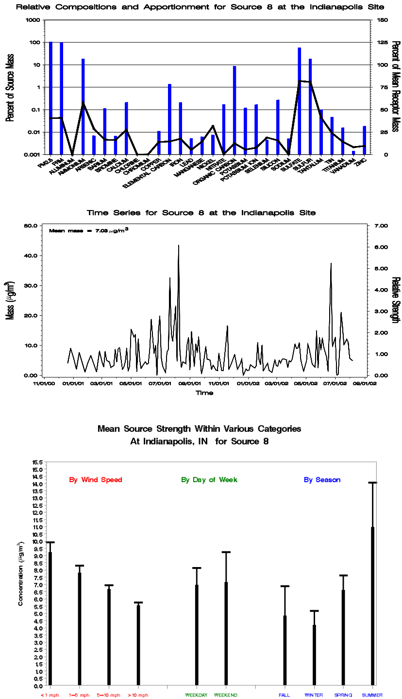
Figure H-43. Profile Plot (Top), Time Series Plot (Middle), and Bar Charts of the Source Strength Averaged by Wind Speed, Day of Week, and Season (Bottom) for Indianapolis, Indiana, Source 8 – Coal Combustion 2 (Ni).
