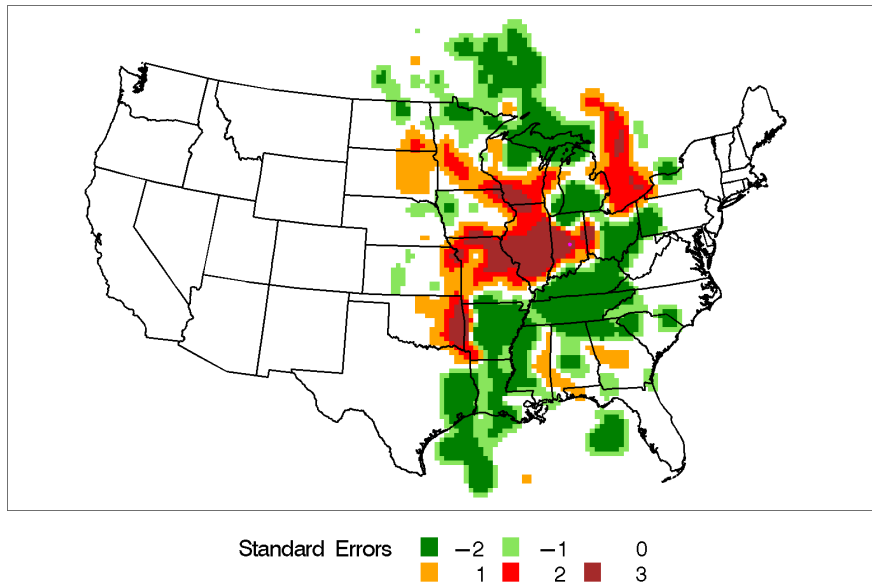
Figure H-10 Incremental Probability Contour Plot for Indianapolis, Indiana, Source 2 – Ammonium Nitrate.
