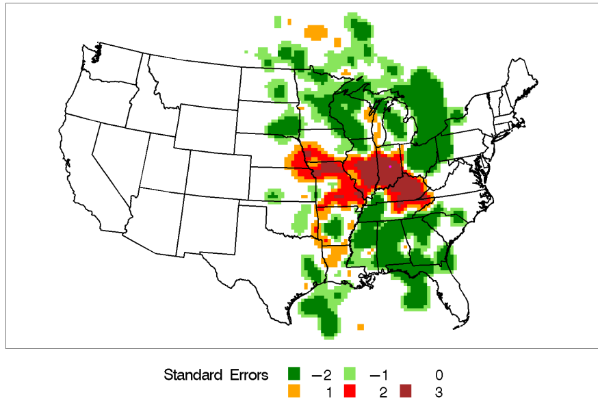
Figure H-40 Incremental Probability Contour Plot for Indianapolis, Indiana, Source 7 – Coal Combustion 1.
