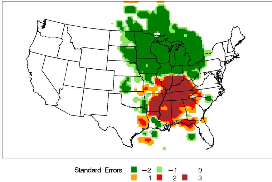
Figure H-46 Incremental Probability Contour Plot for Indianapolis, Indiana, Source 8 – Coal Combustion 2 (Ni).
