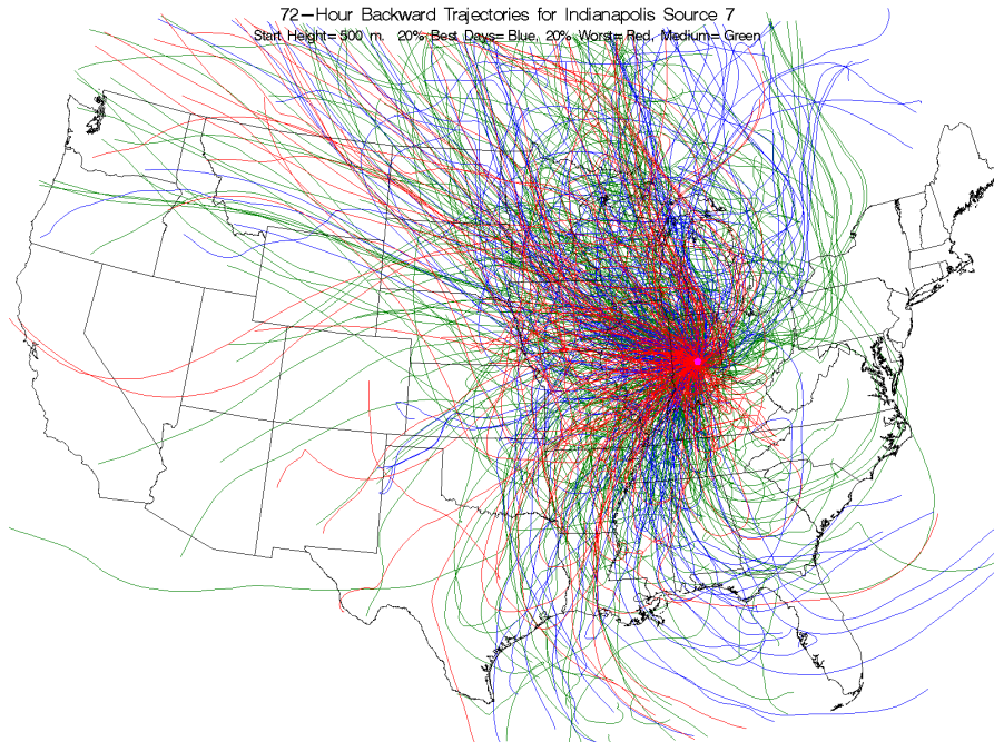
Figure H-41 Back Trajectories Color Coded by Source Strength Category for Indianapolis, Indiana, Source 7 – Coal Combustion 1.
